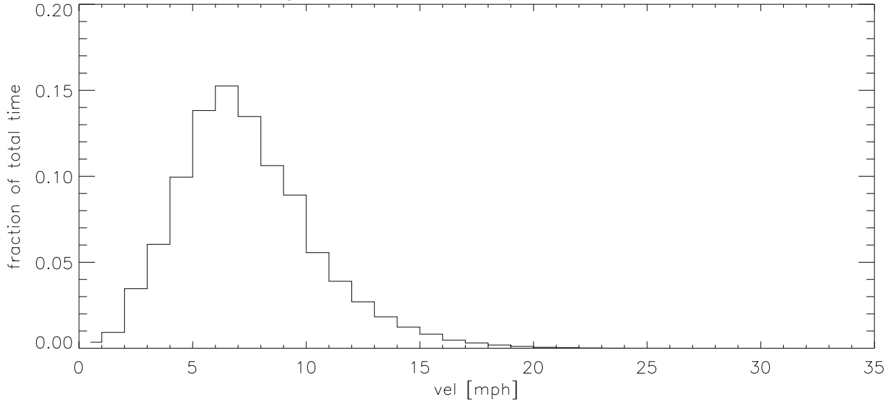
DEC11 Fraction of time wind velocity exceeds specified vel
