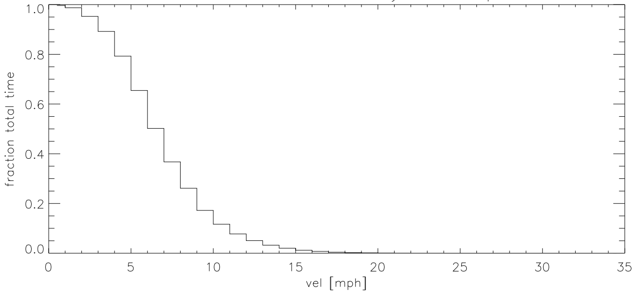
DEC11 Fraction of time wind velocity exceeds specified vel (blowup)
