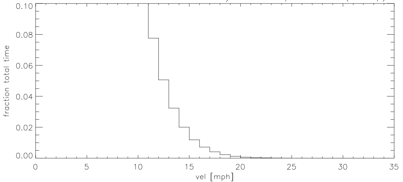
DEC11 Fraction of time wind velocity exceeds specified vel (blowup)
