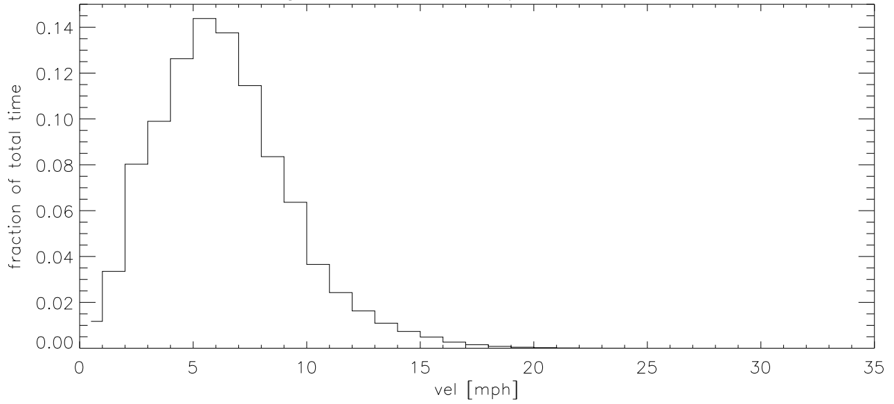
NOV11 Fraction of time wind velocity exceeds specified vel
