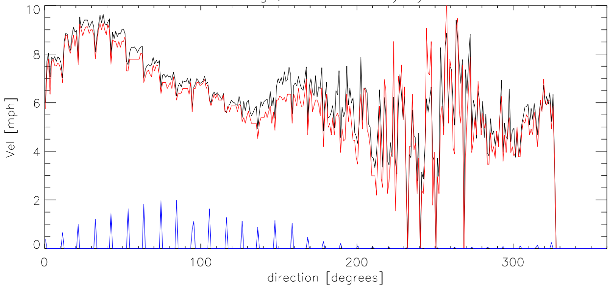
NOV11 Average, median velocity by direction
