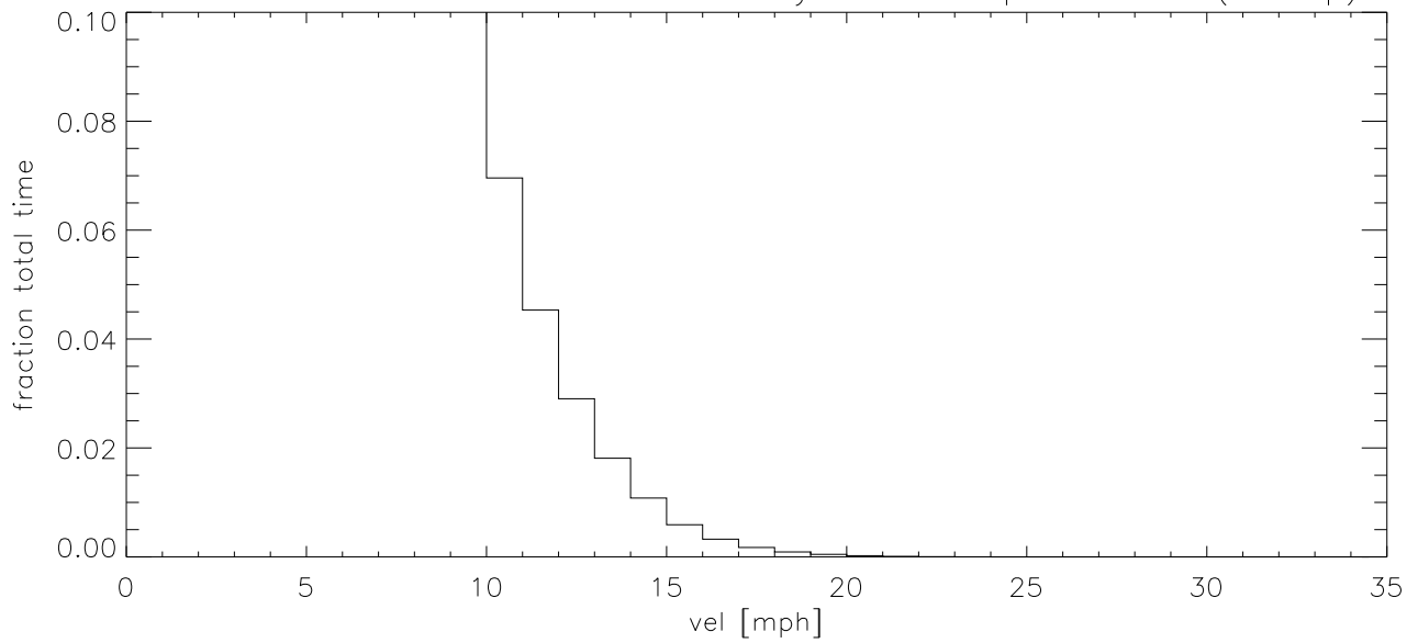
NOV11 Fraction of time wind velocity exceeds specified vel (blowup)
