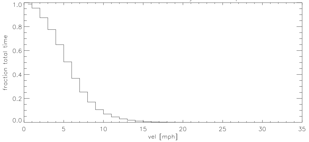
NOV11 Fraction of time wind velocity exceeds specified vel (blowup)
