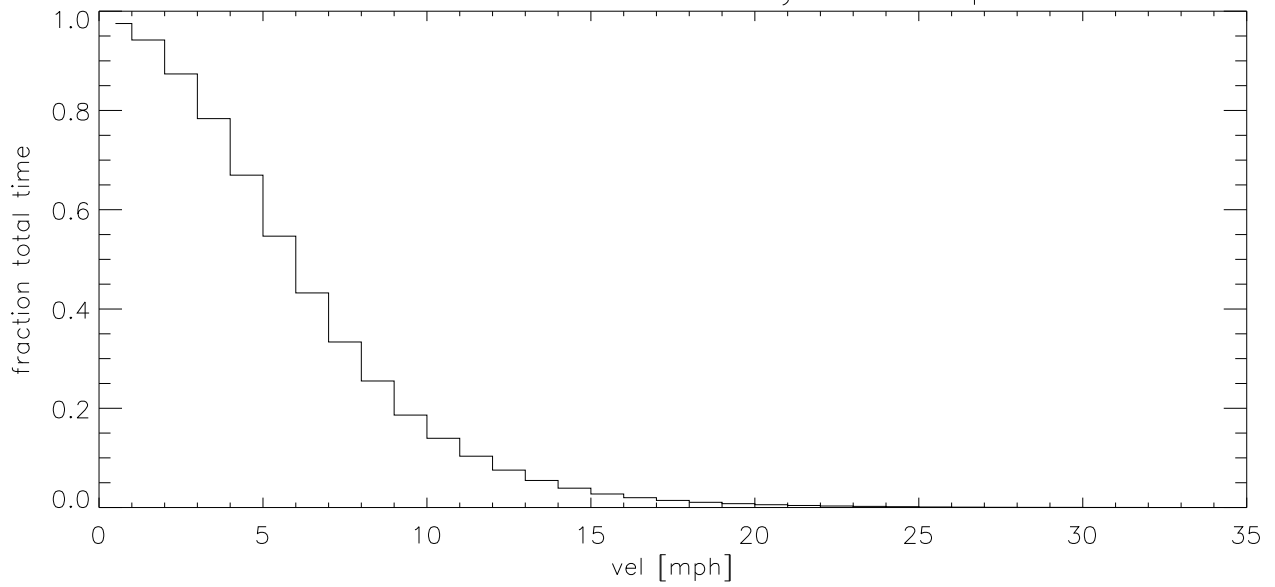
AUG11 Fraction of time wind velocity exceeds specified vel (blowup)
