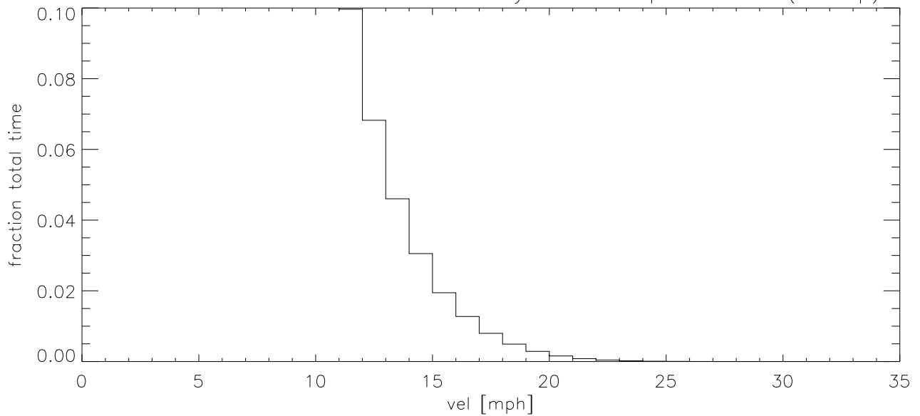
FEB11 Fraction of time wind velocity exceeds specified vel (blowup)
