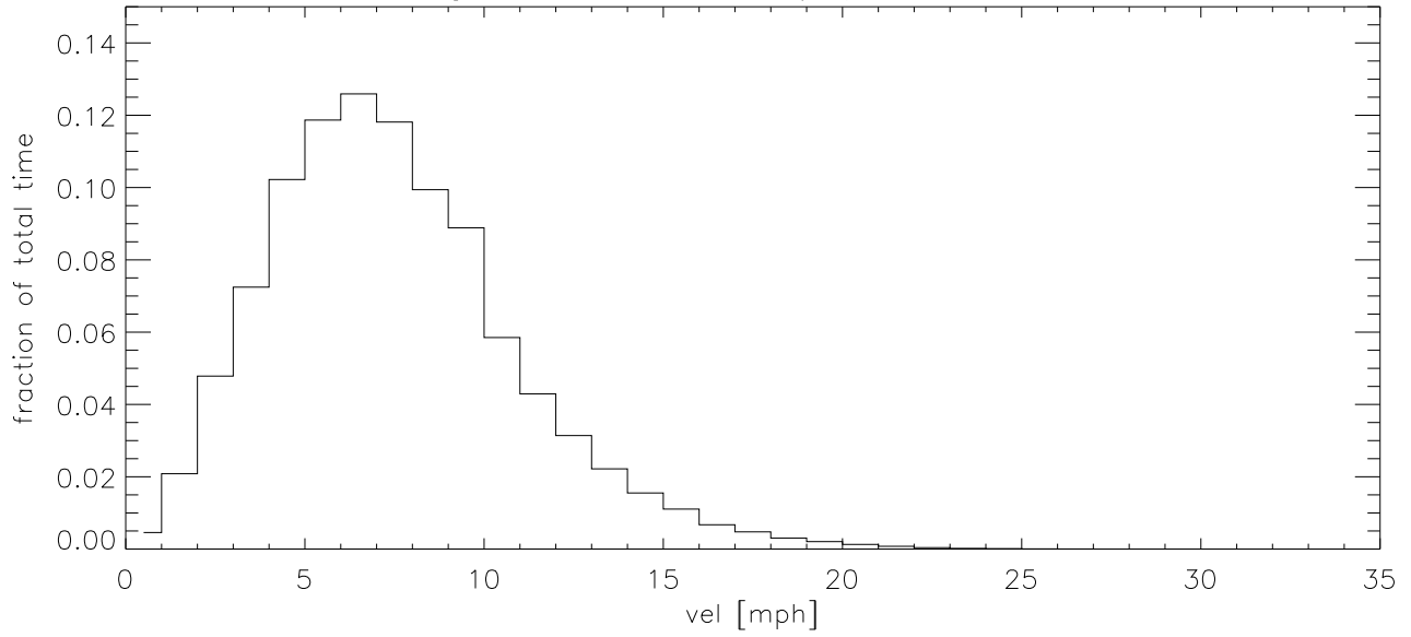
FEB11 Fraction of time wind velocity exceeds specified vel
