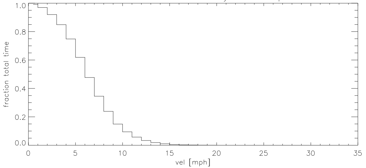
JAN11 Fraction of time wind velocity exceeds specified vel (blowup)
