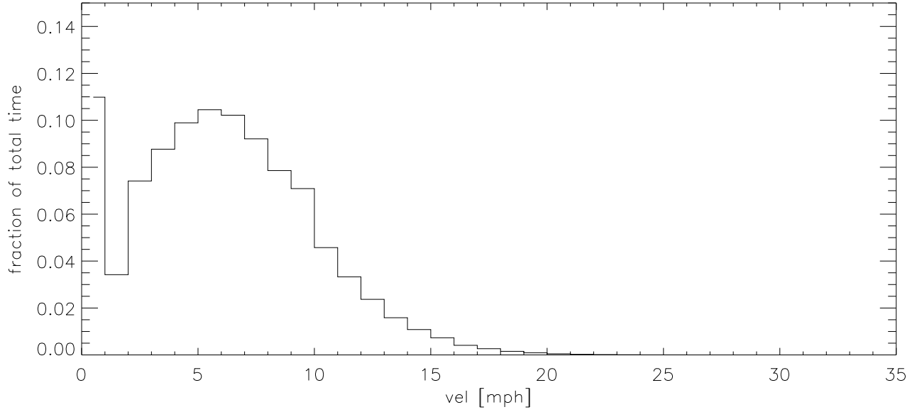
APR09 Fraction of time wind velocity exceeds specified vel
