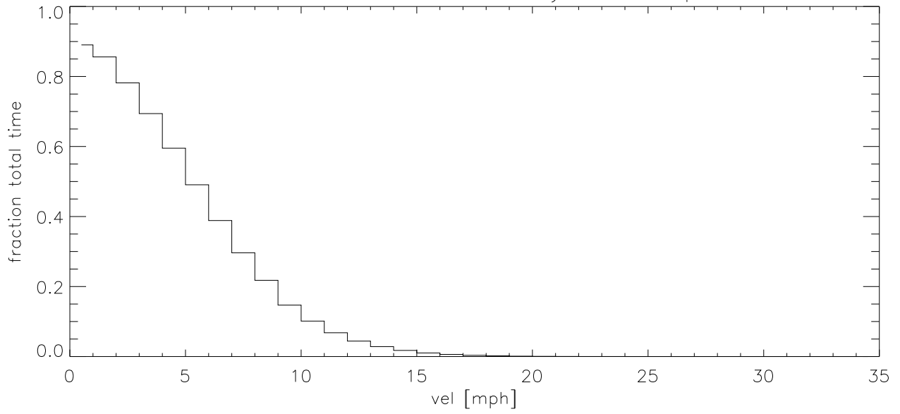
APR09 Fraction of time wind velocity exceeds specified vel (blowup)
