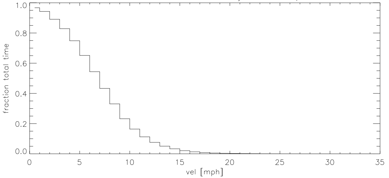
JUN08 Fraction of time wind velocity exceeds specified vel (blowup)
