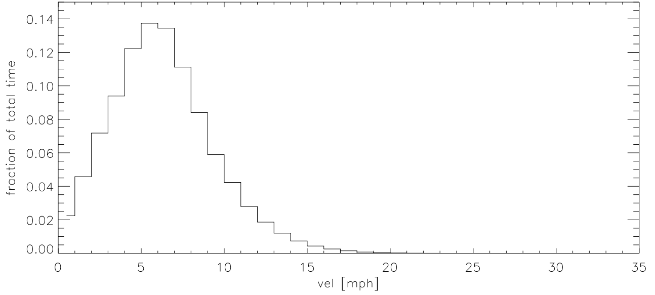
NOV07 Fraction of time wind velocity exceeds specified vel
