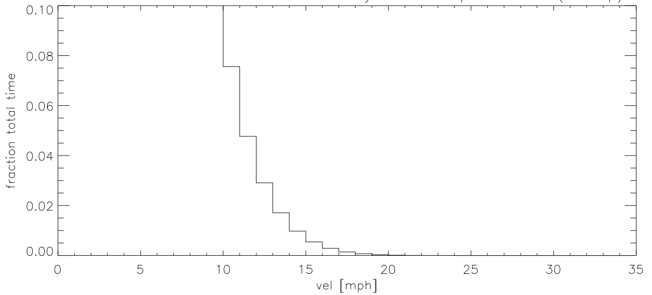
NOV07 Fraction of time wind velocity exceeds specified vel (blowup)
