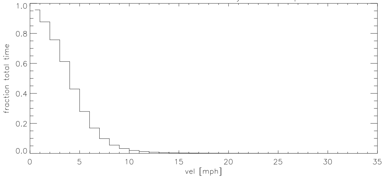
AUG05 Fraction of time wind velocity exceeds specified vel (blowup)
