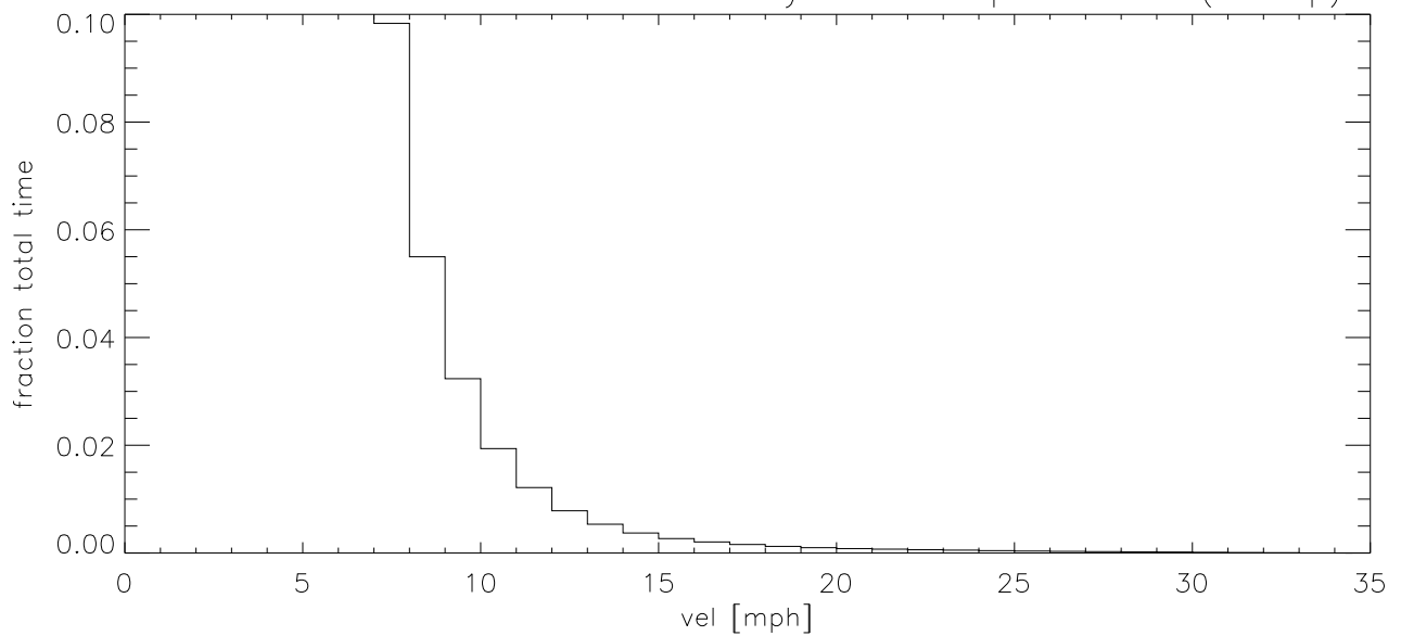
AUG05 Fraction of time wind velocity exceeds specified vel (blowup)
