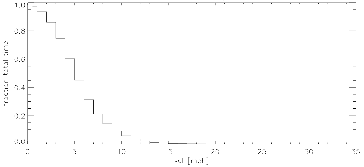
MAY05 Fraction of time wind velocity exceeds specified vel (blowup)
