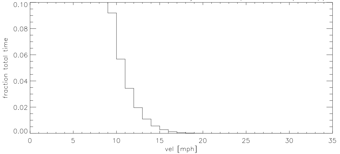
MAY05 Fraction of time wind velocity exceeds specified vel (blowup)
