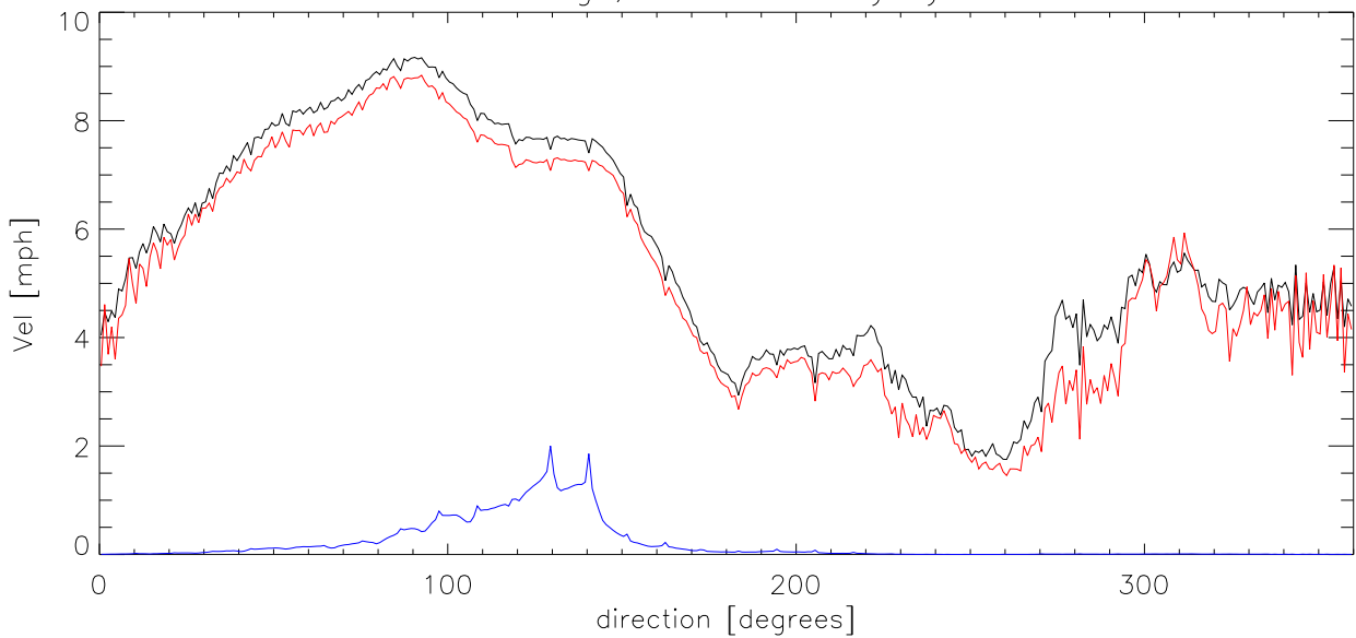
JUL03 Average, median velocity by direction
