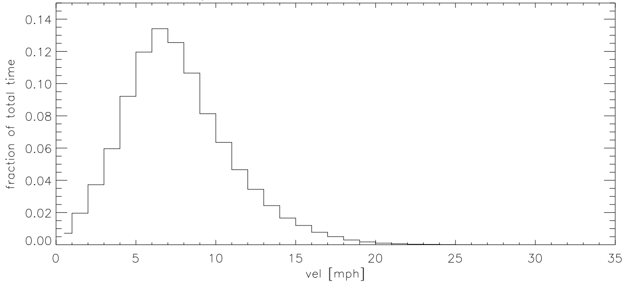
JUL03 Fraction of time wind velocity exceeds specified vel
