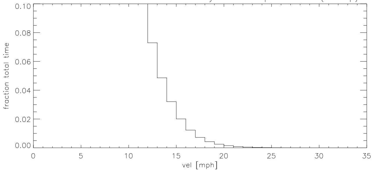
JUL03 Fraction of time wind velocity exceeds specified vel (blowup)
