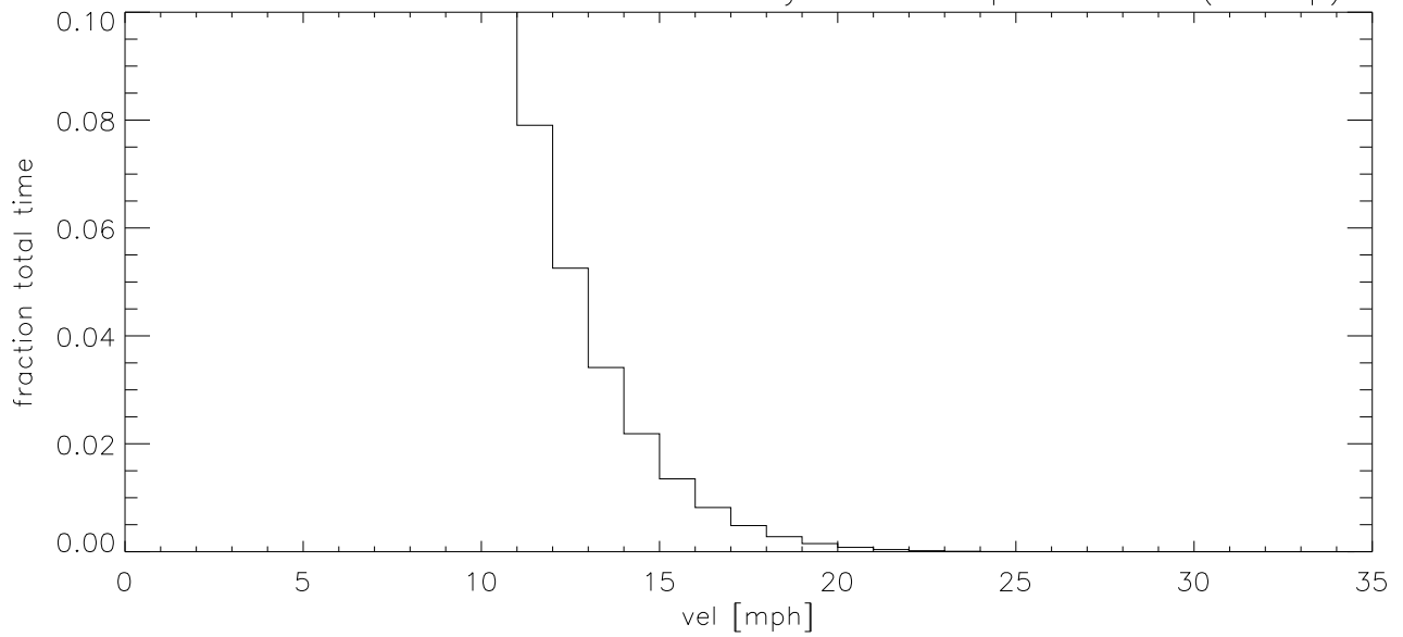
FEB03 Fraction of time wind velocity exceeds specified vel (blowup)
