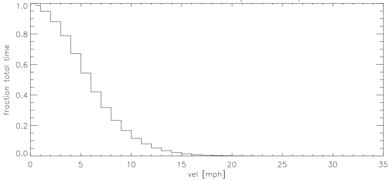
FEB03 Fraction of time wind velocity exceeds specified vel (blowup)
