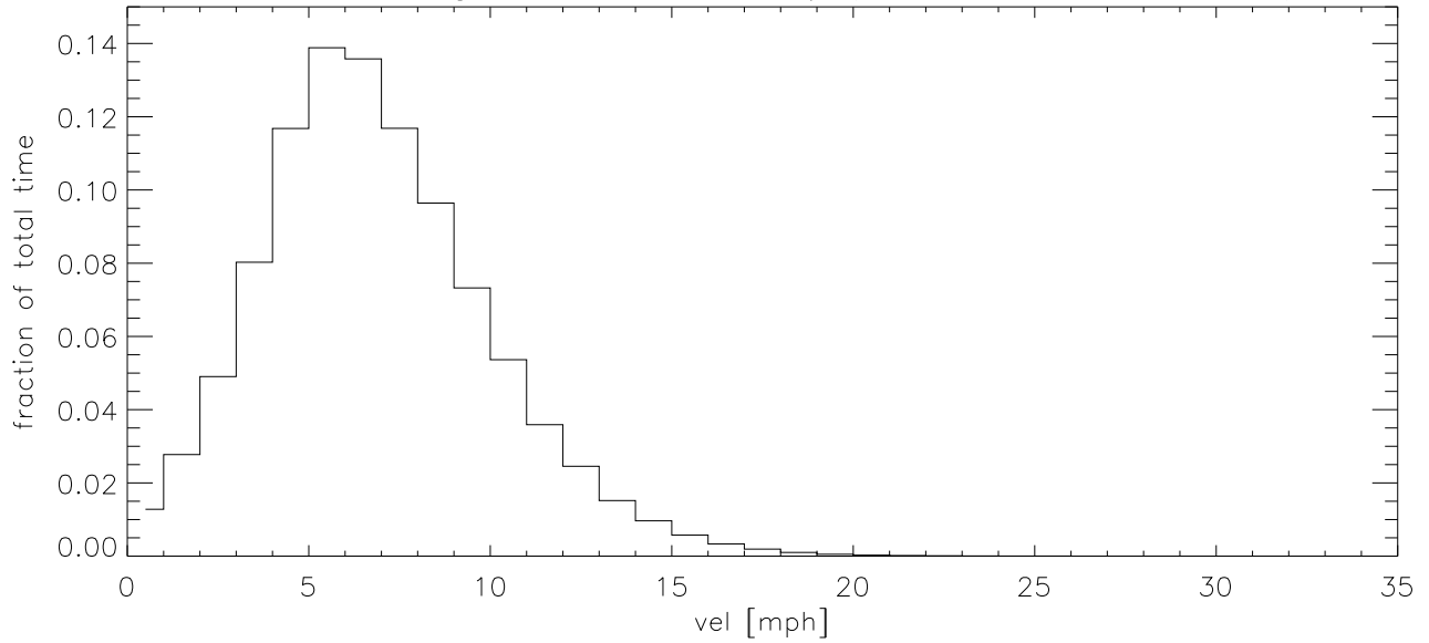
JUL02 Fraction of time wind velocity exceeds specified vel
