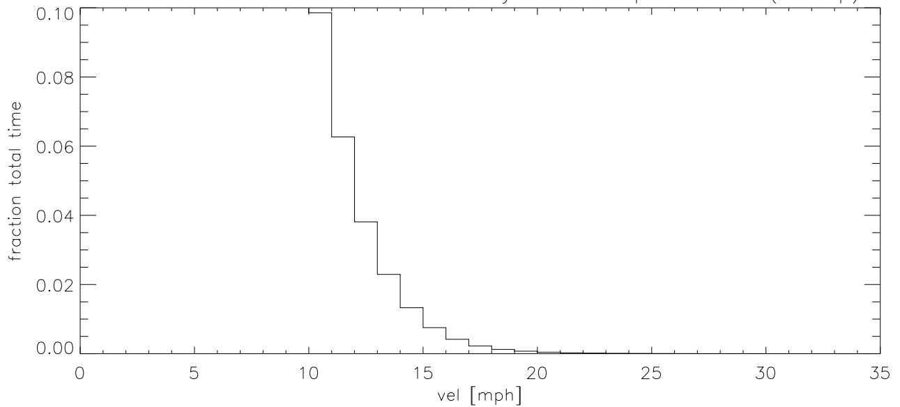
JUL02 Fraction of time wind velocity exceeds specified vel (blowup)
