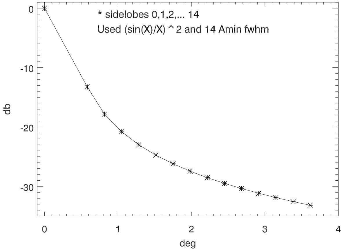
simulation of 327rcvr sidelobe loss vs sidelobe offset
