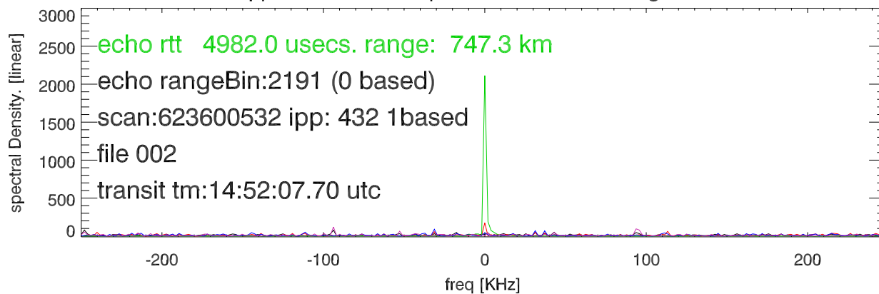
ipp:3000, 5 dcded spectra around echo range 2554
