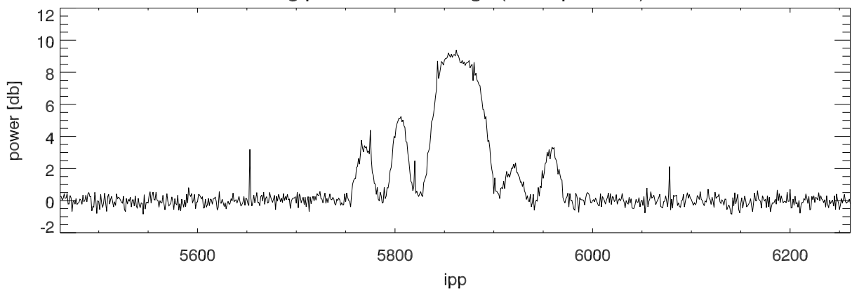
Avg power in echo range (blowup in time)
