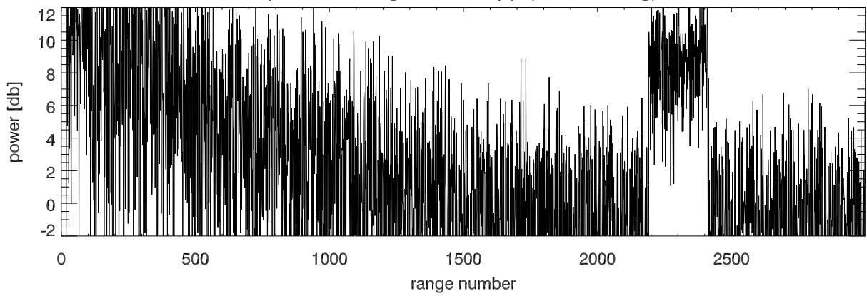
Avg power in echo range vs ipp (no decoding)
