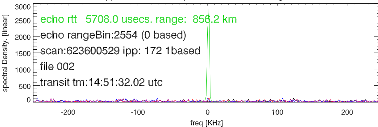
ipp:3000, 5 dced spectra around echo range 2554
