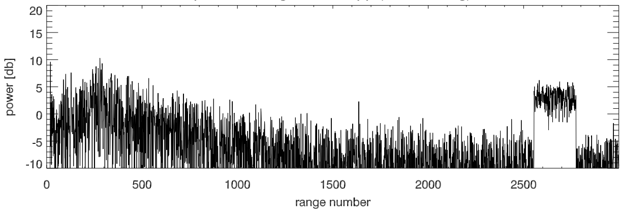
Avg power in echo range vs ipp (no decoding)
