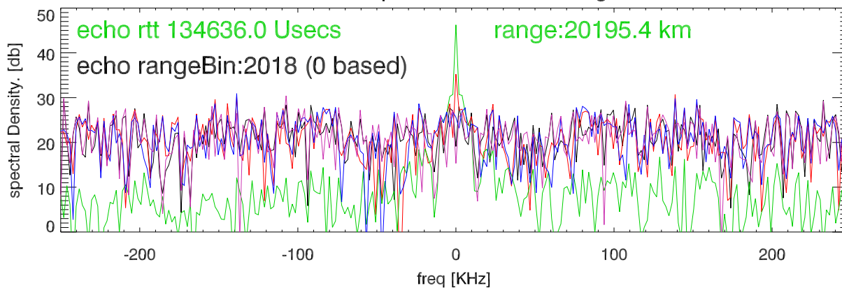
5 dced spectra around echo range
