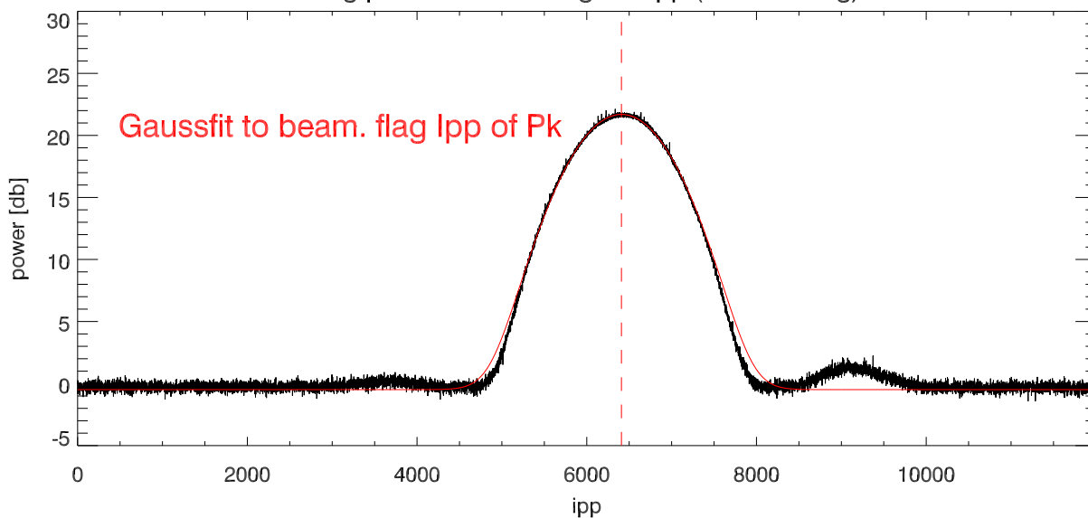
Avg power in echo range vs lpp (no decoding)
