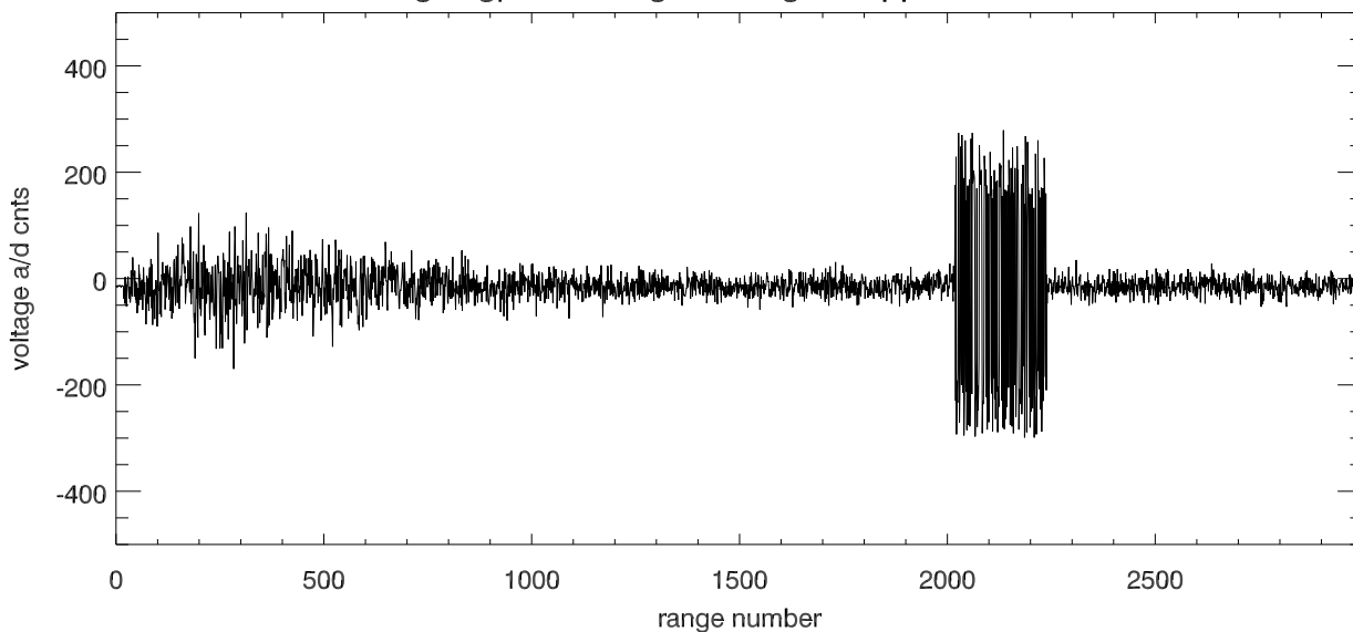
23aug16 gps01 Voltage vs range for ipp with max echo
