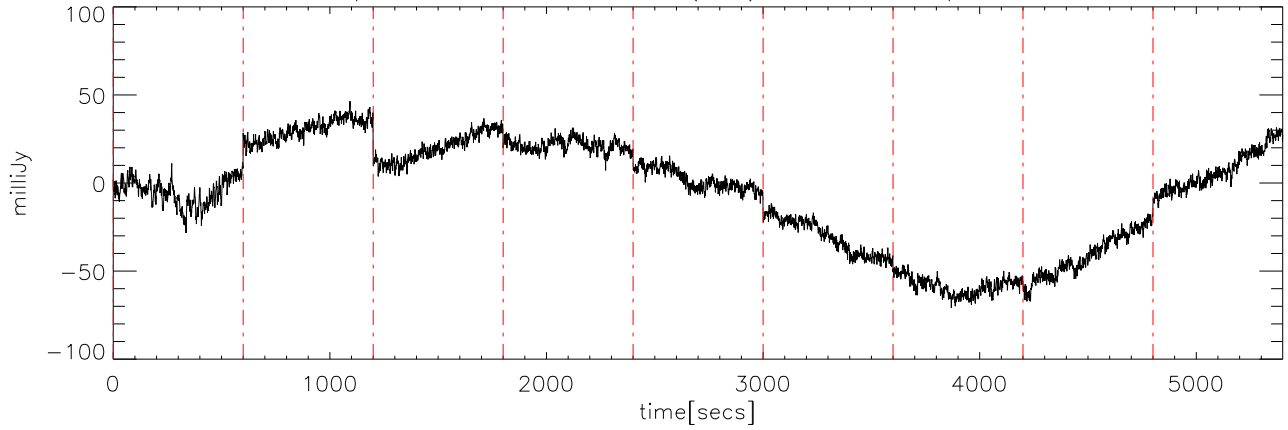
p2111 file:12 30dec08 (AST) StokesQ freq:5250.
