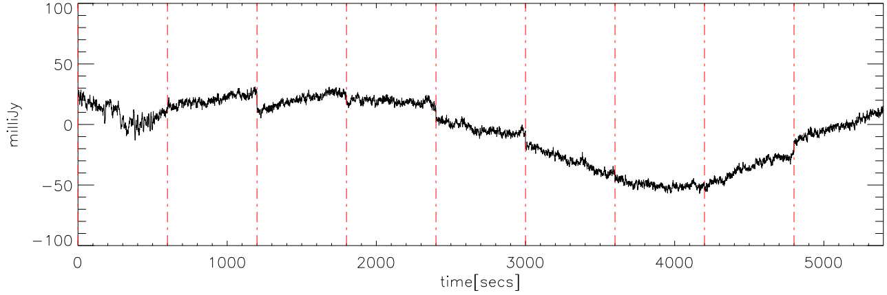
p2111 file:12 30dec08 (AST) StokesQ freq:5000.
