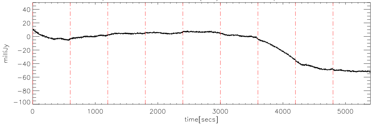
p2111 file:12 30dec08 (AST) StokesU freq:4600.
