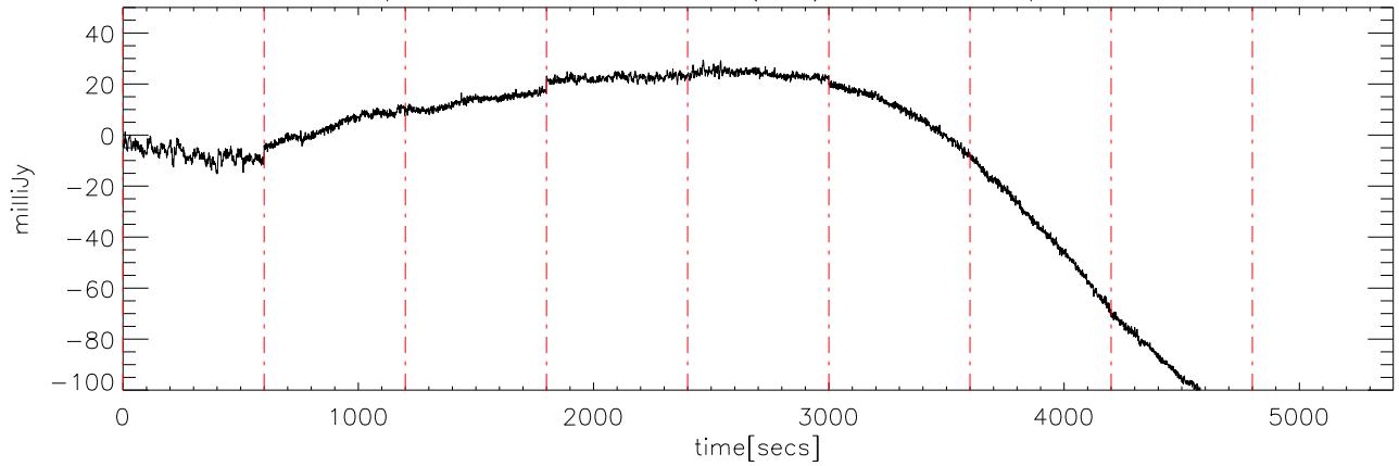
p2111 file:12 30dec08 (AST) StokesU freq:5250.
