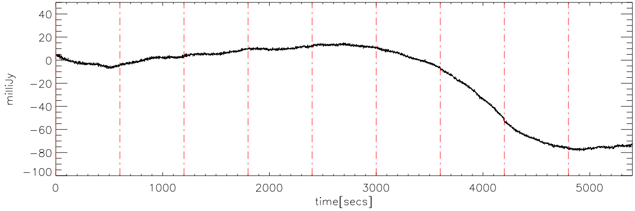
p2111 file:12 30dec08 (AST) StokesU freq:5000.
