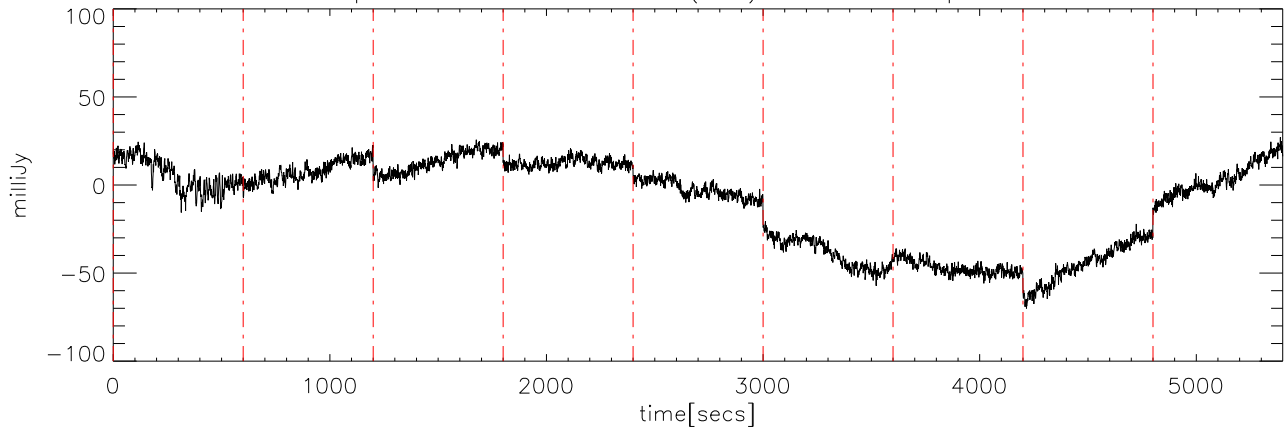
p2111 file:12 30dec08 (AST) StokesQ freq:5125.
