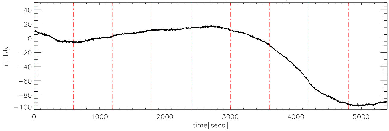
p2111 file:12 30dec08 (AST) StokesU freq:5125.
