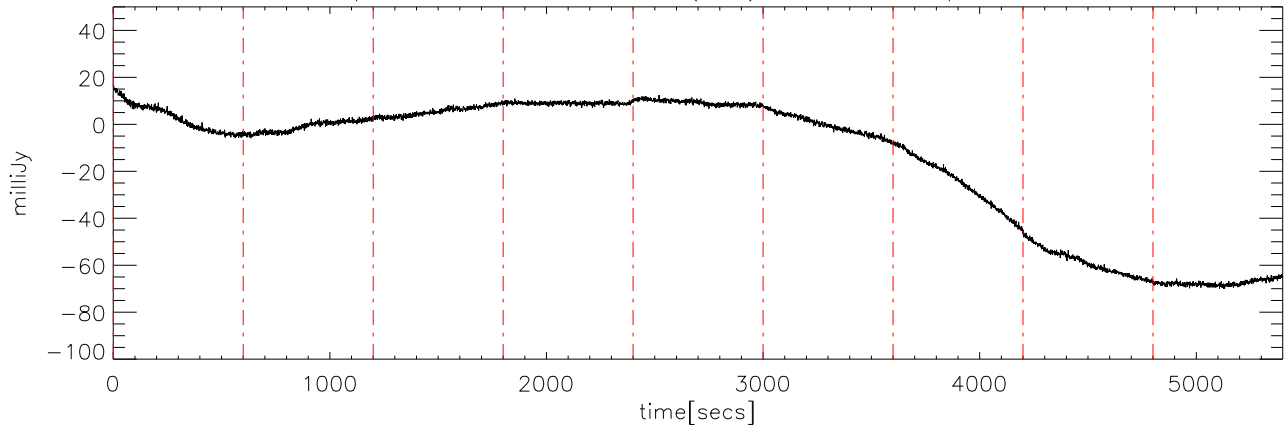
p2111 file:12 30dec08 (AST) StokesU freq:4725.
