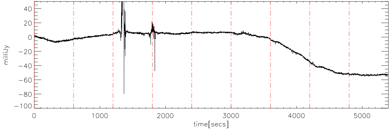
p2111 file:12 30dec08 (AST) StokesU freq:4475.
