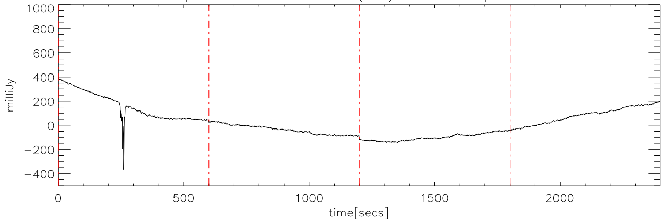
p2111 file:04 30dec08 (AST) StokesI freq:5250.
