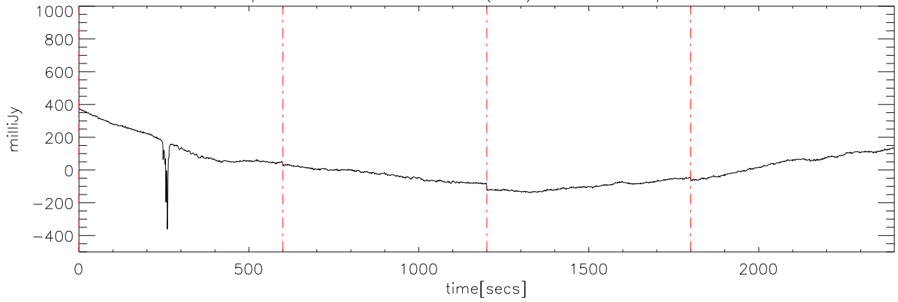
p2111 file:04 30dec08 (AST) StokesI freq:5125.
