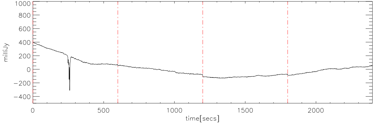
p2111 file:04 30dec08 (AST) StokesI freq:5000.
