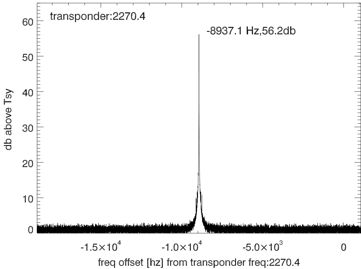
isee3 140627:195406 (UTC) spectra after doppler correction. PolA
