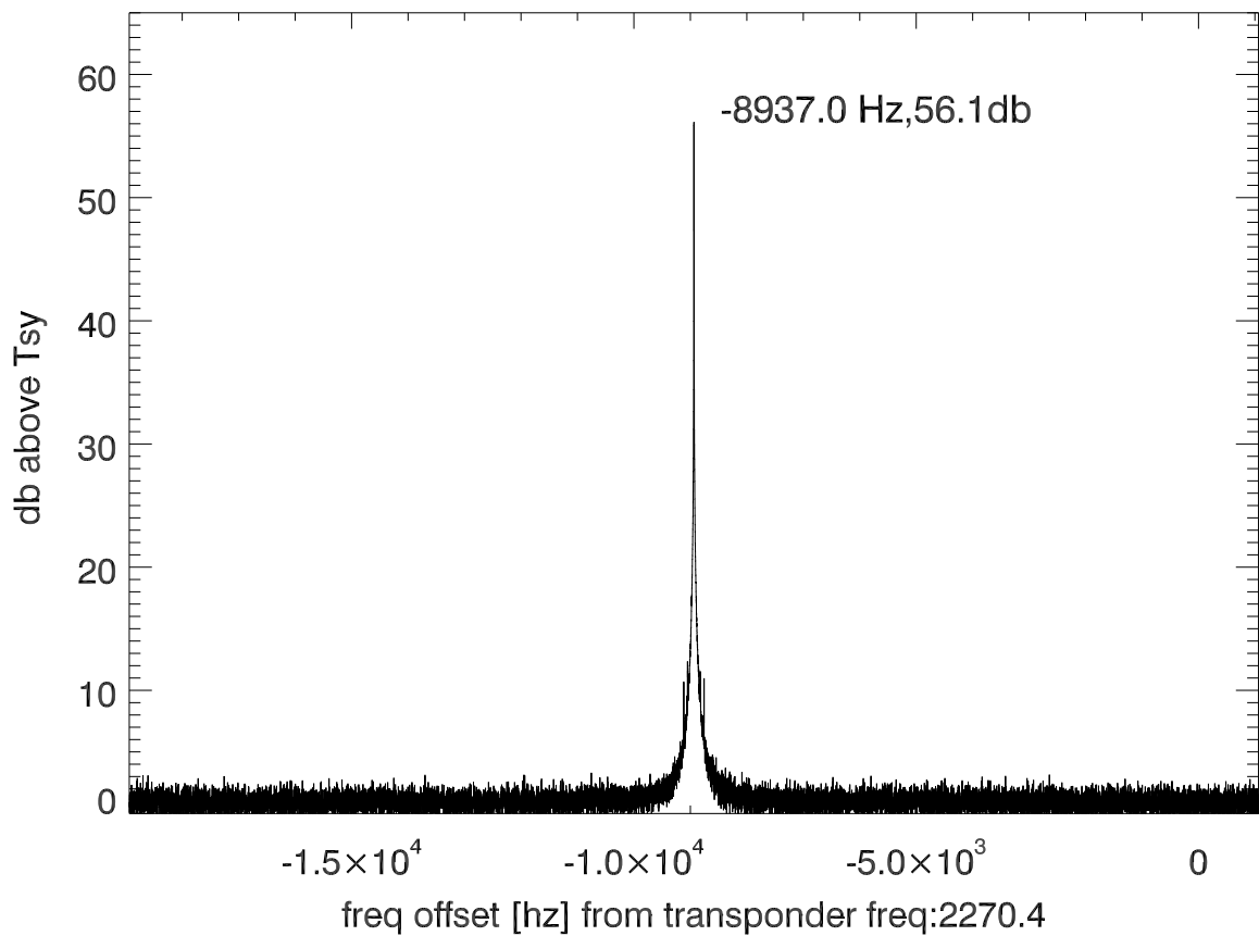
isee3 140627:195406 (UTC) spectra after doppler correction. PolB
