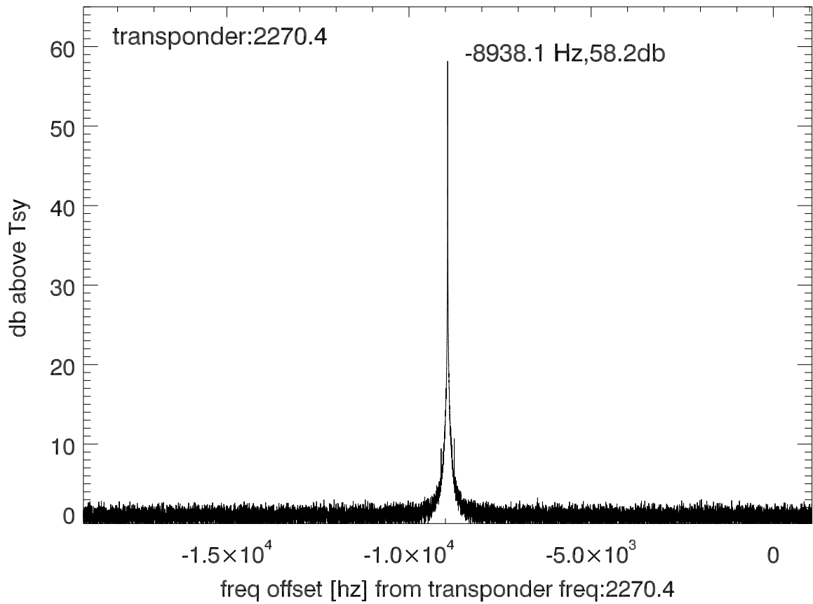
isee3 140627:193852 (UTC) spectra after doppler correction. PolA
