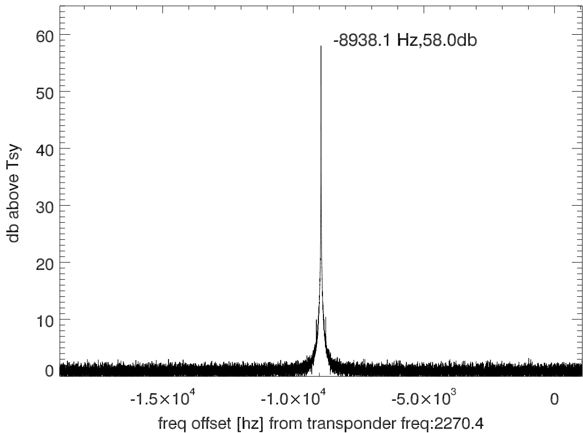
isee3 140627:193852 (UTC) spectra after doppler correction. PolB
