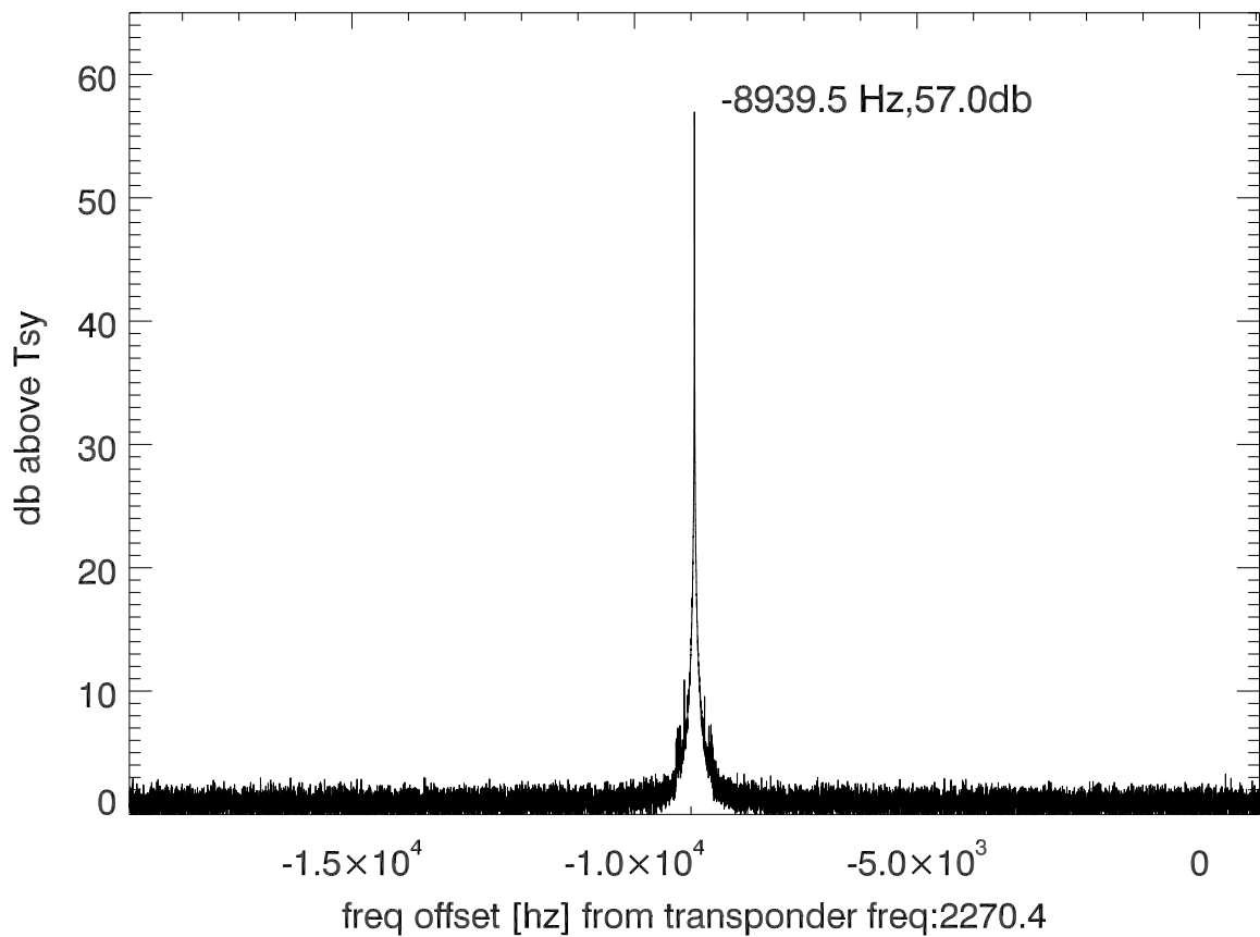
isee3 140627:191814 (UTC) spectra after doppler correction. PolB
