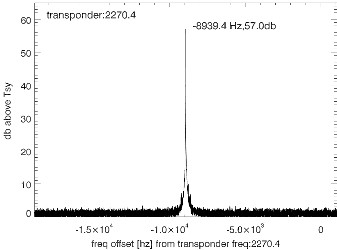
isee3 140627:191814 (UTC) spectra after doppler correction. PolA
