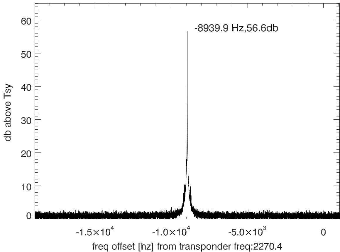
isee3 140627:185809 (UTC) spectra after doppler correction. PolB
