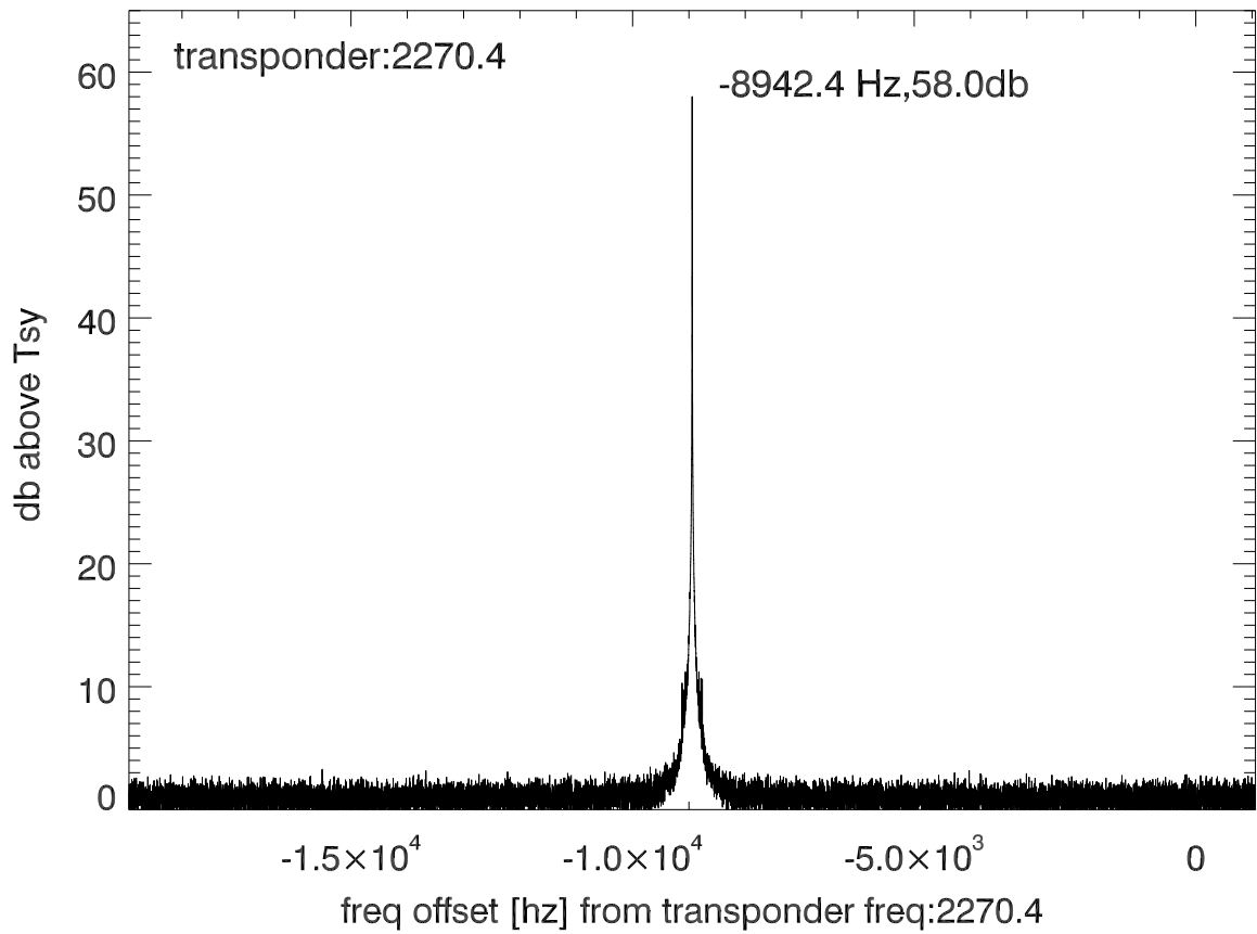
isee3 140627:182444 (UTC) spectra after doppler correction. PolA
