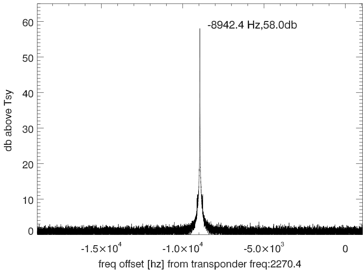
isee3 140627:182444 (UTC) spectra after doppler correction. PolB
