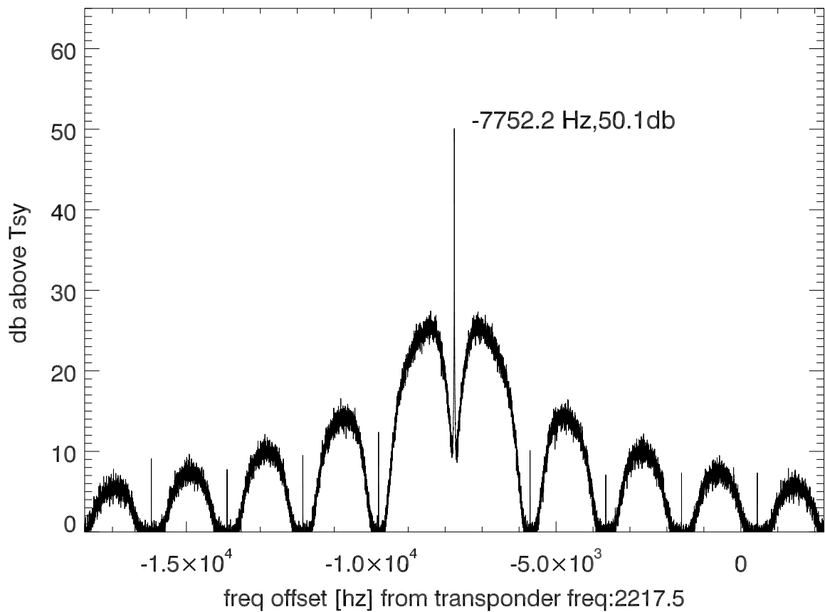
isee3 140627:193605 (UTC) spectra after doppler correction. PoIB
