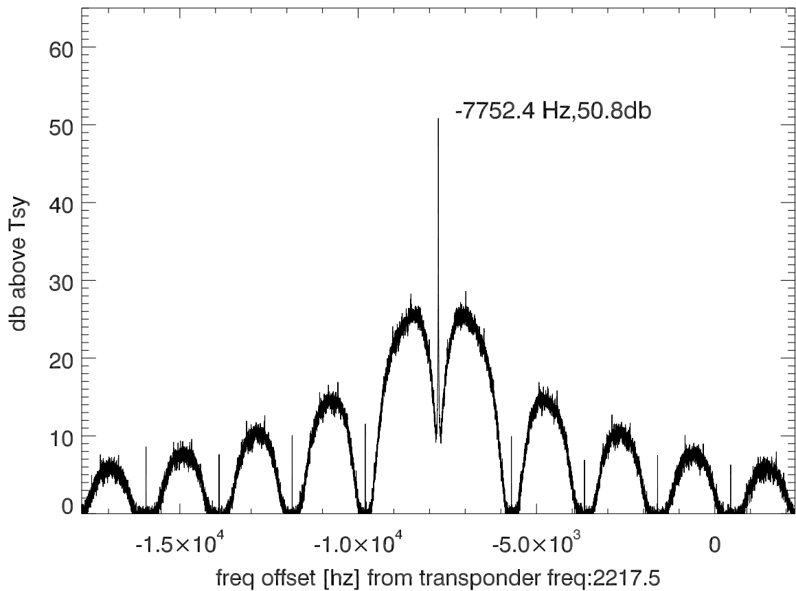
isee3 140627:192629 (UTC) spectra after doppler correction. PoIB
