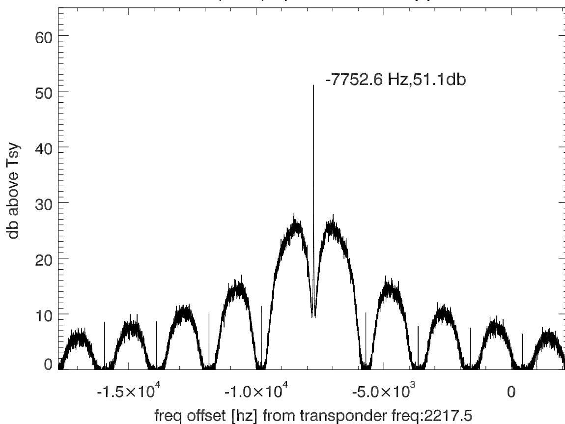
isee3 140627:192349 (UTC) spectra after doppler correction. PoIB
