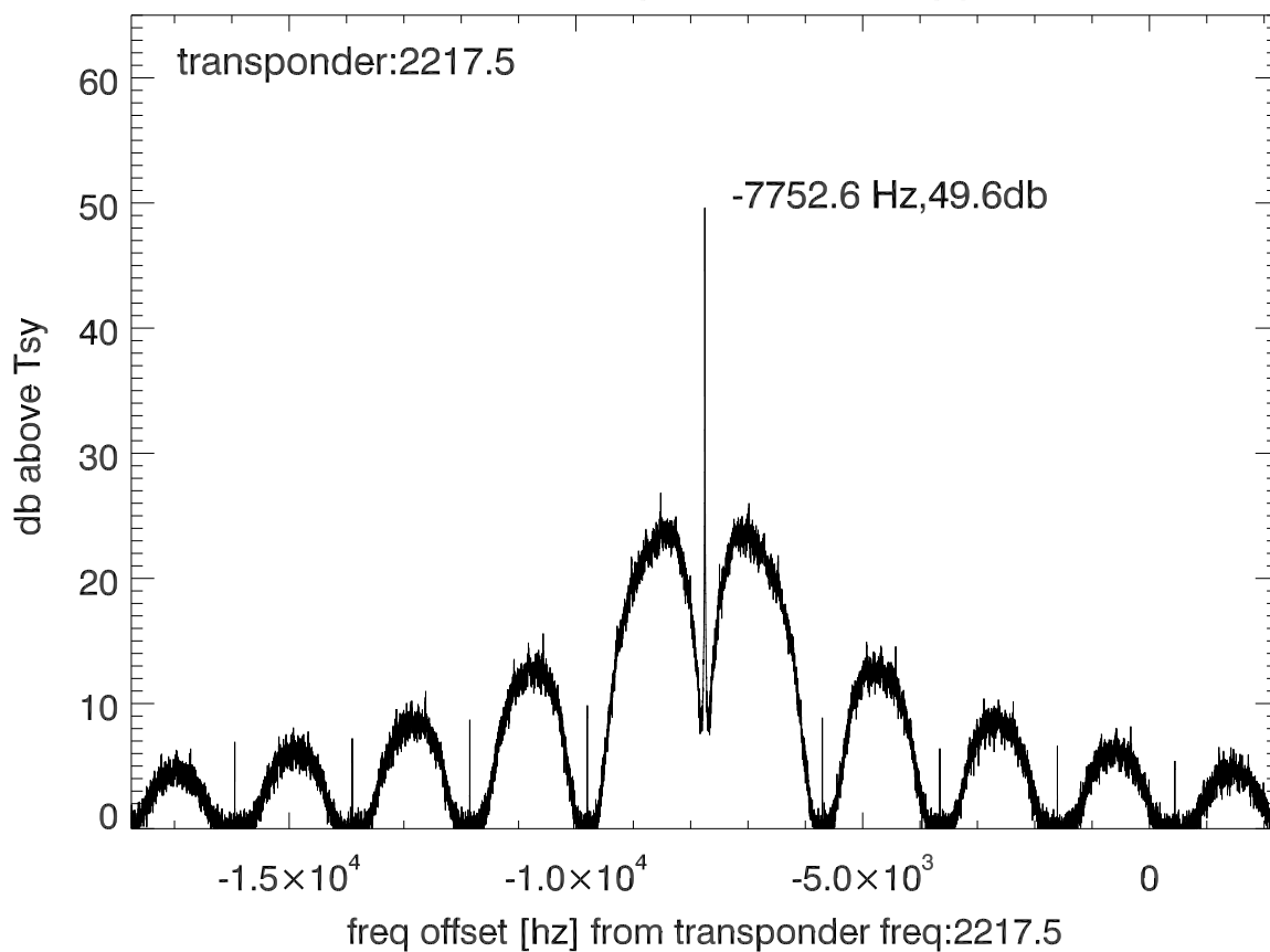
isee3 140627:192349 (UTC) spectra after doppler correction. PoIA
