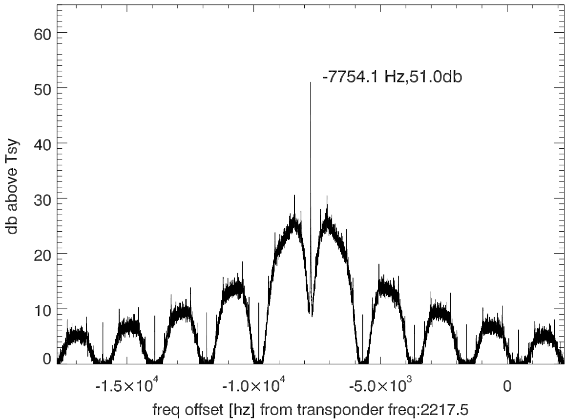
isee3 140627:182715 (UTC) spectra after doppler correction. PoIB
