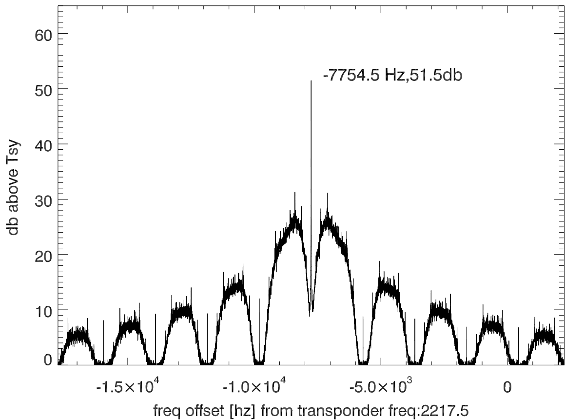
isee3 140627:180618 (UTC) spectra after doppler correction. PoIB
