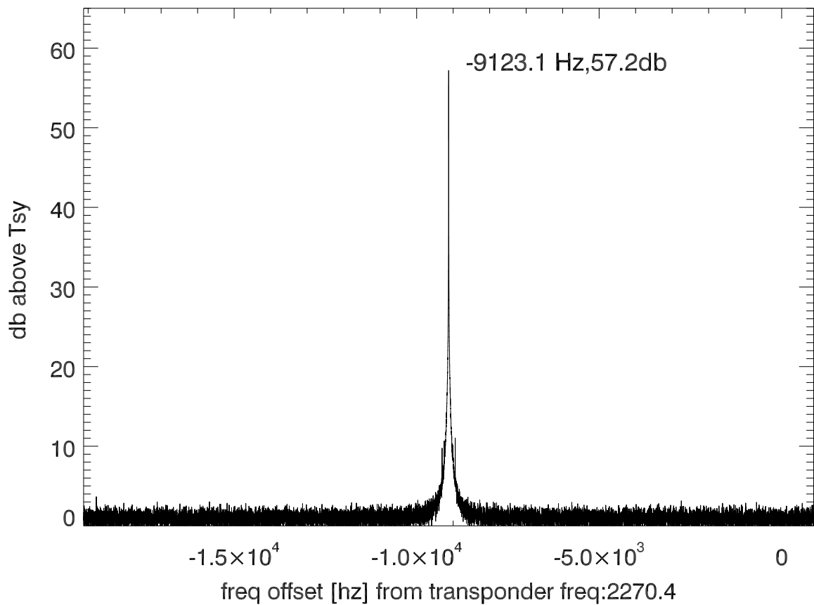
isee3 140625:175052 (UTC) spectra after doppler correction. PolB
