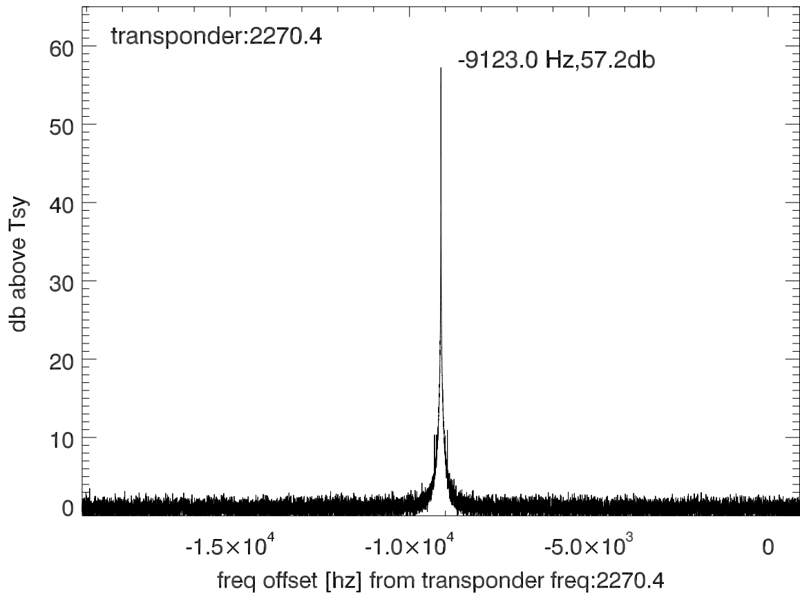
isee3 140625:175052 (UTC) spectra after doppler correction. PolA
