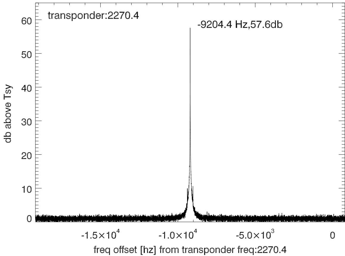
isee3 140624:195626 (UTC) spectra after doppler correction. PolA
