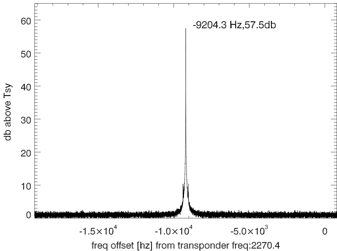
isee3 140624:195626 (UTC) spectra after doppler correction. PolB
