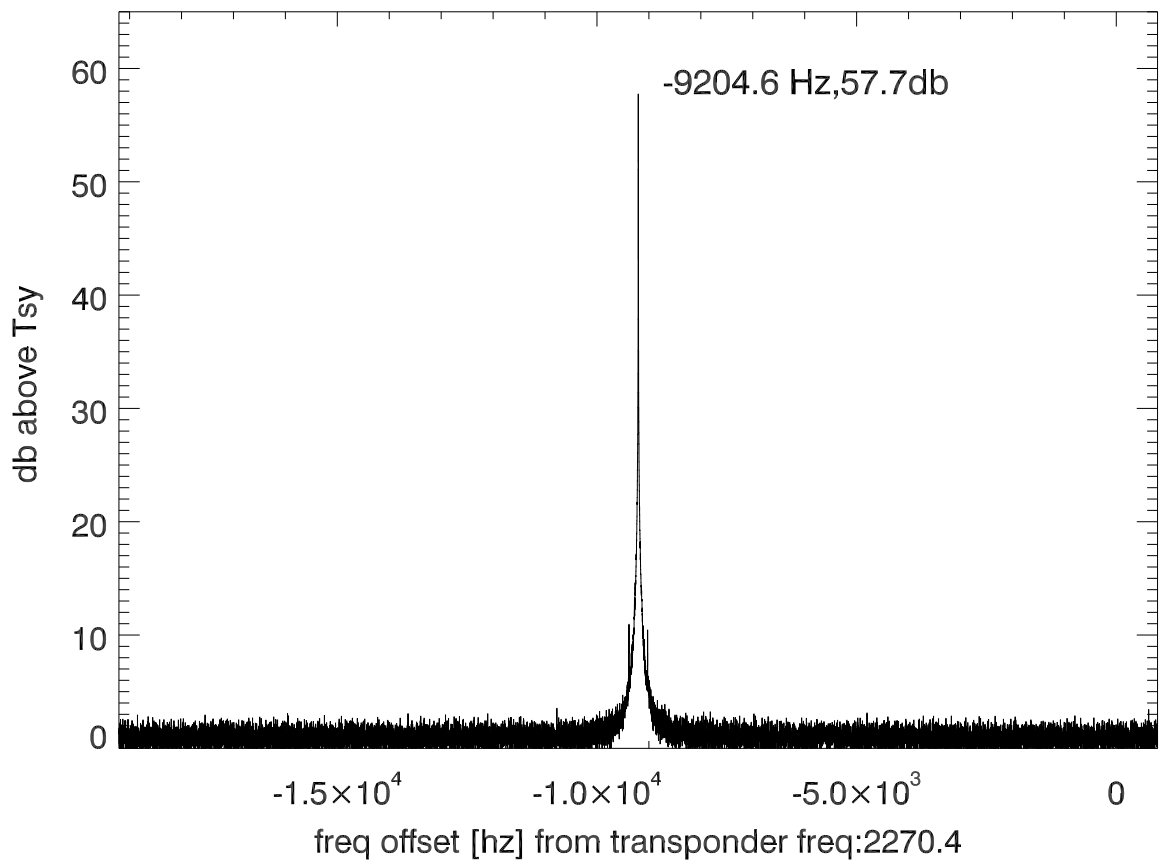
isee3 140624:195427 (UTC) spectra after doppler correction. PolB
