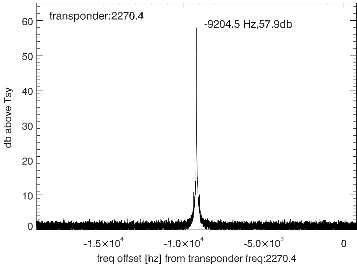
isee3 140624:195427 (UTC) spectra after doppler correction. PolA
