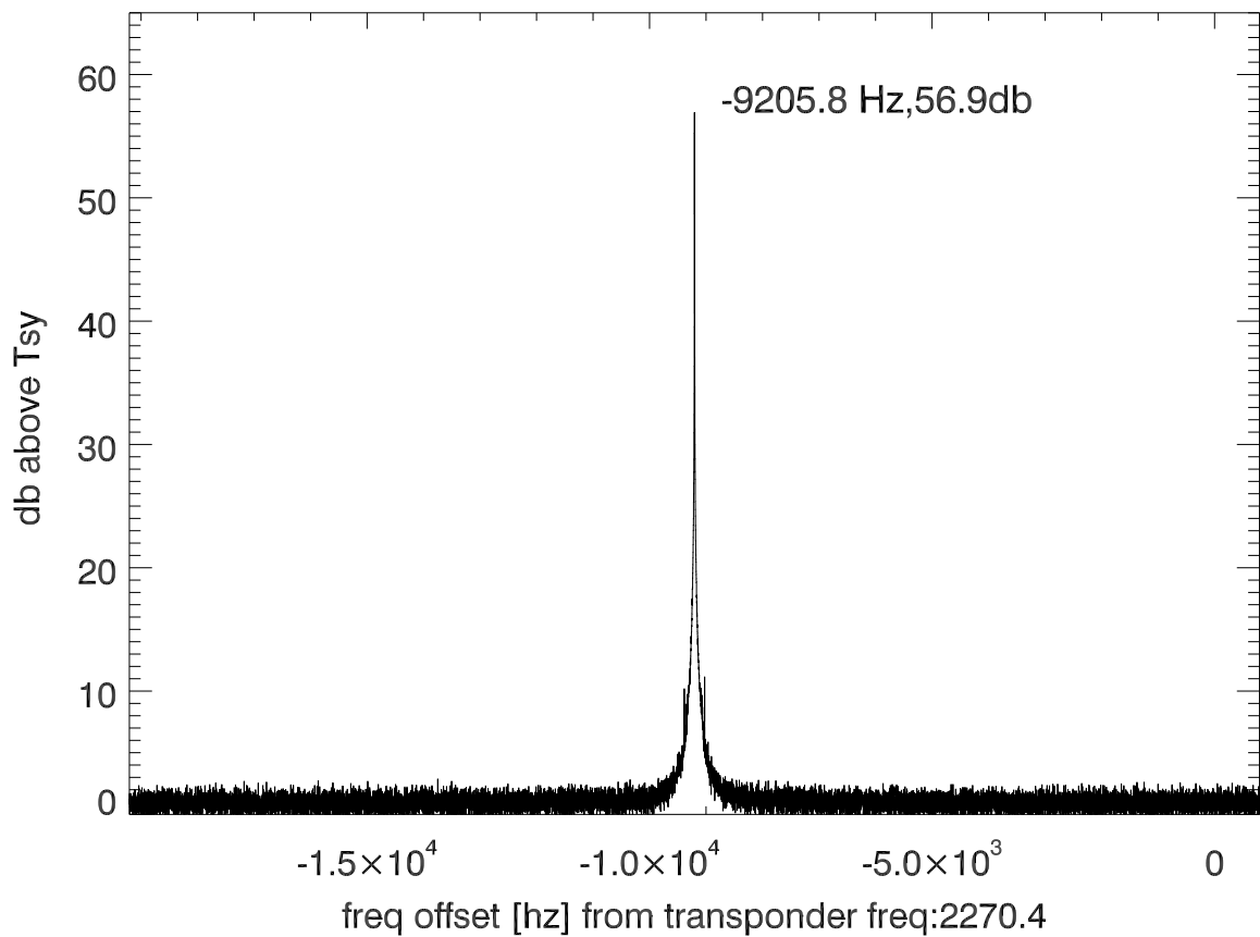
isee3 140624:193730 (UTC) spectra after doppler correction. PolB
