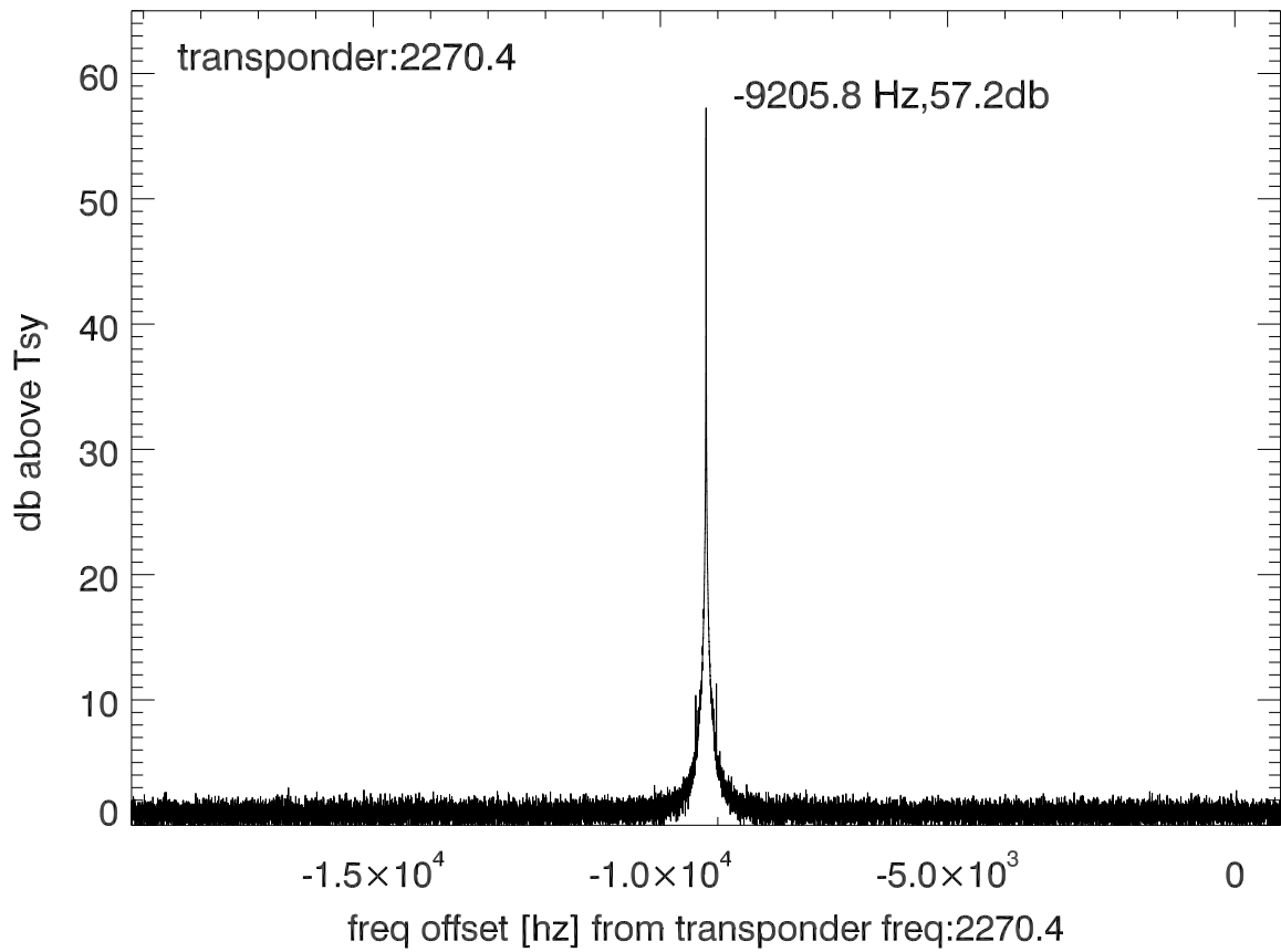
isee3 140624:193730 (UTC) spectra after doppler correction. PolA
