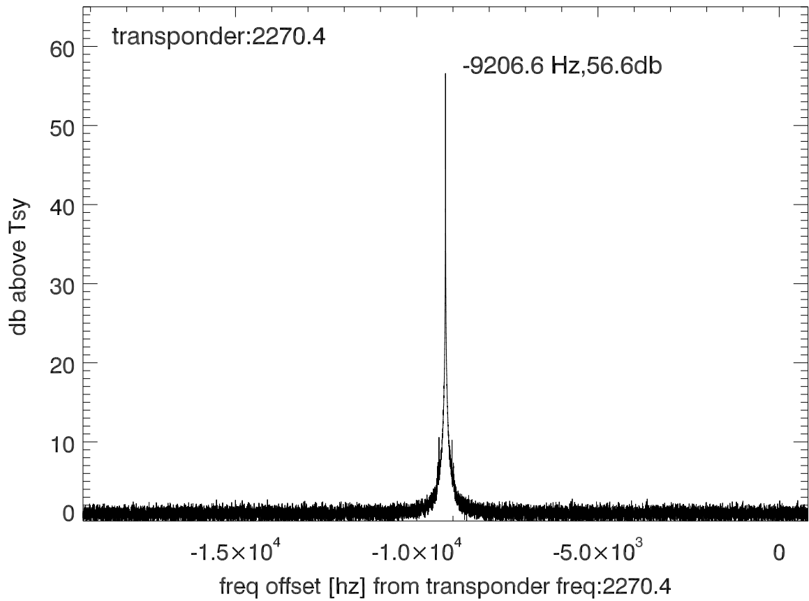
isee3 140624:192315 (UTC) spectra after doppler correction. PolA
