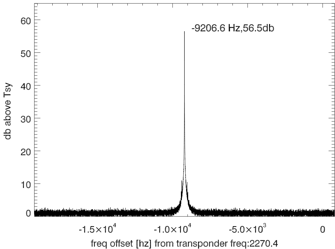
isee3 140624:192315 (UTC) spectra after doppler correction. PolB
