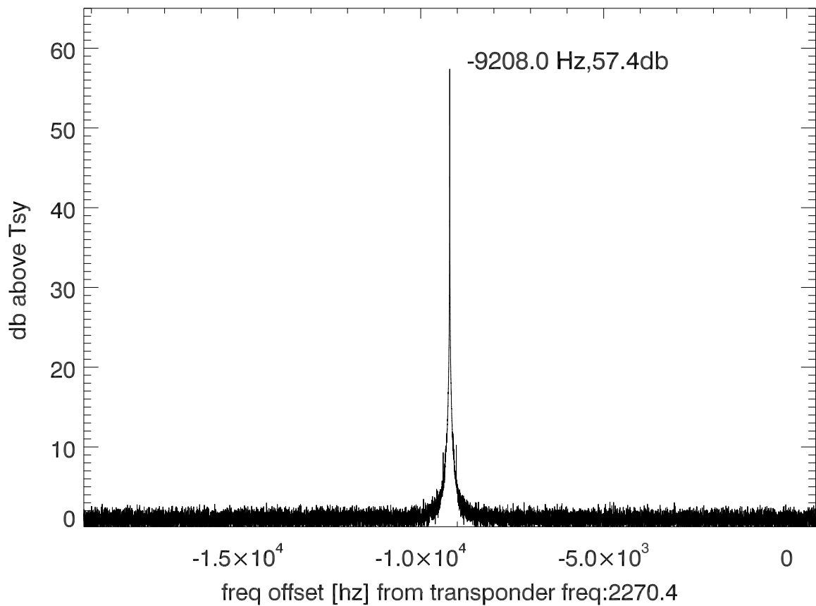
isee3 140624:190723 (UTC) spectra after doppler correction. PolB
