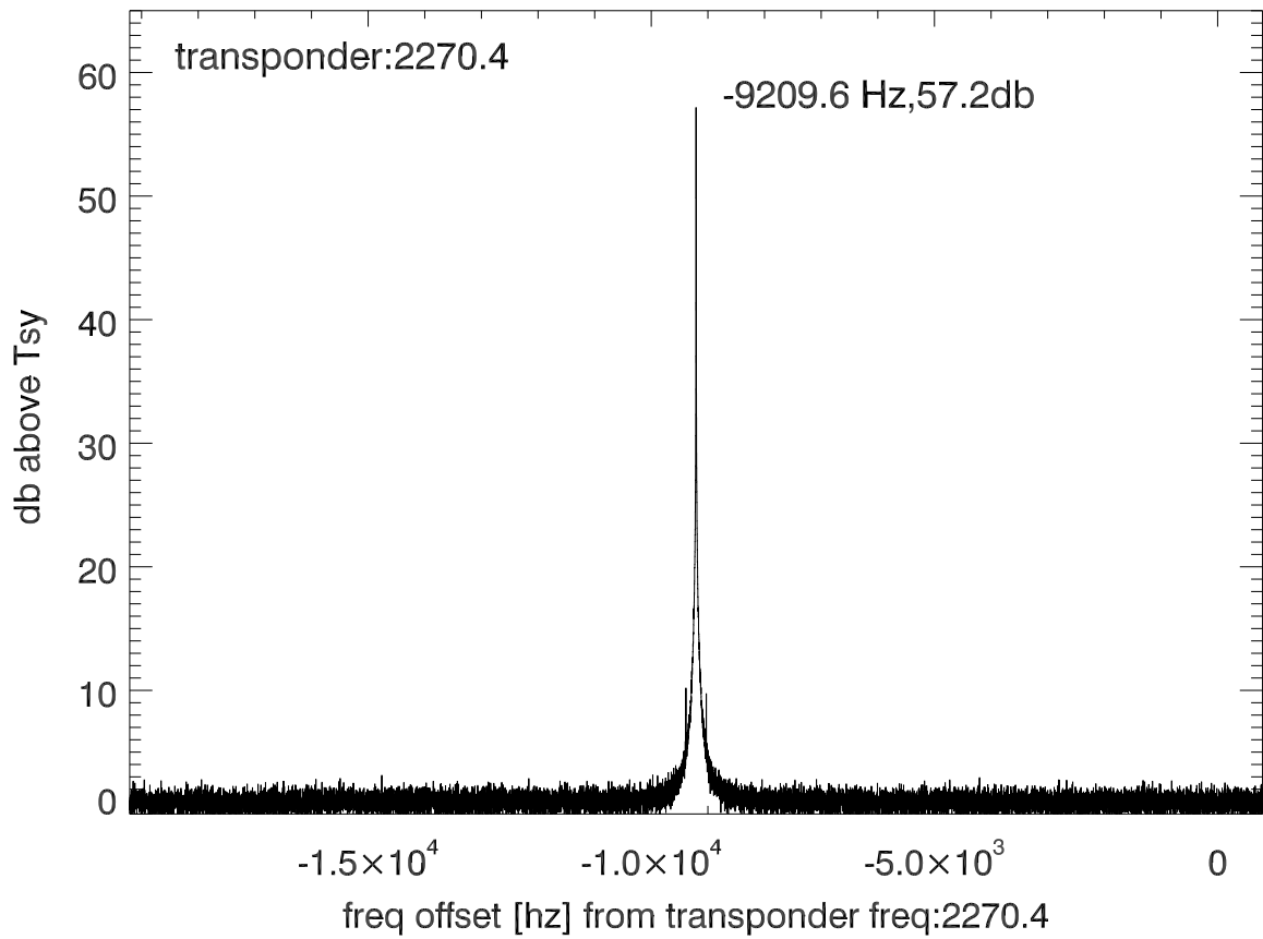
isee3 140624:190235 (UTC) spectra after doppler correction. PolA
