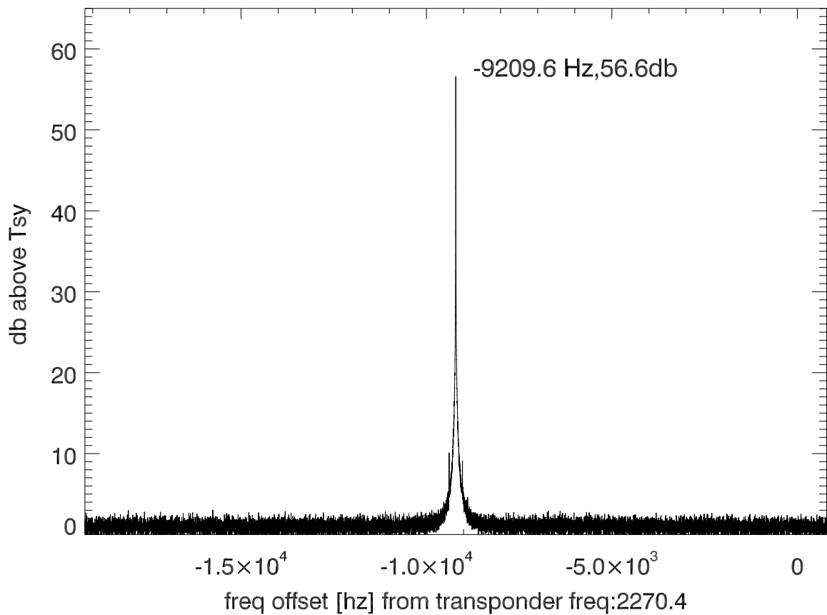
isee3 140624:190235 (UTC) spectra after doppler correction. PolB
