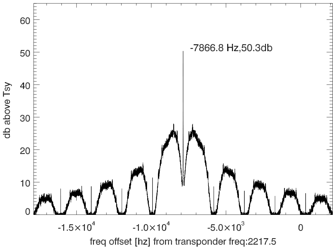
isee3 140624:195626 (UTC) spectra after doppler correction. PoIB
