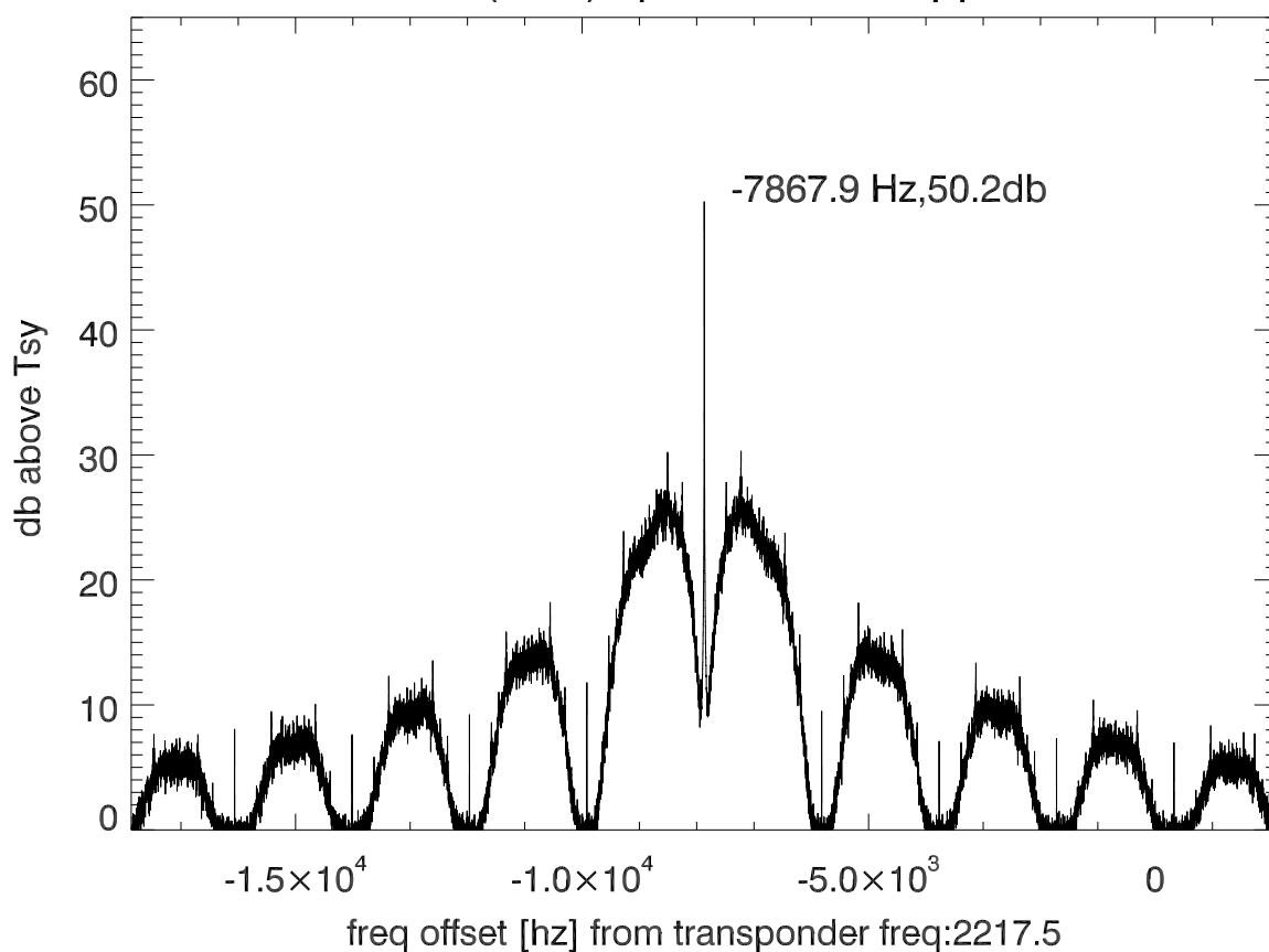
isee3 140624:191729 (UTC) spectra after doppler correction. PoIB
