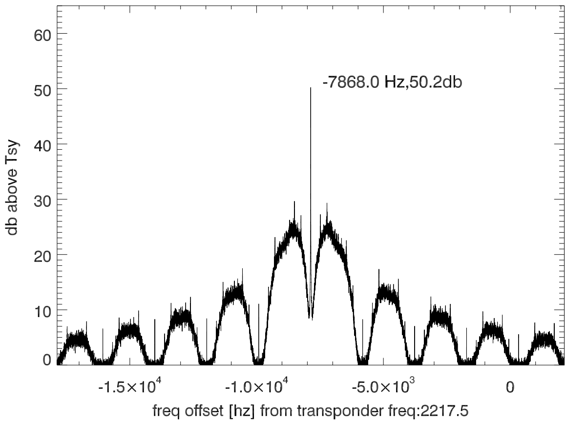
isee3 140624:190235 (UTC) spectra after doppler correction. PoIB
