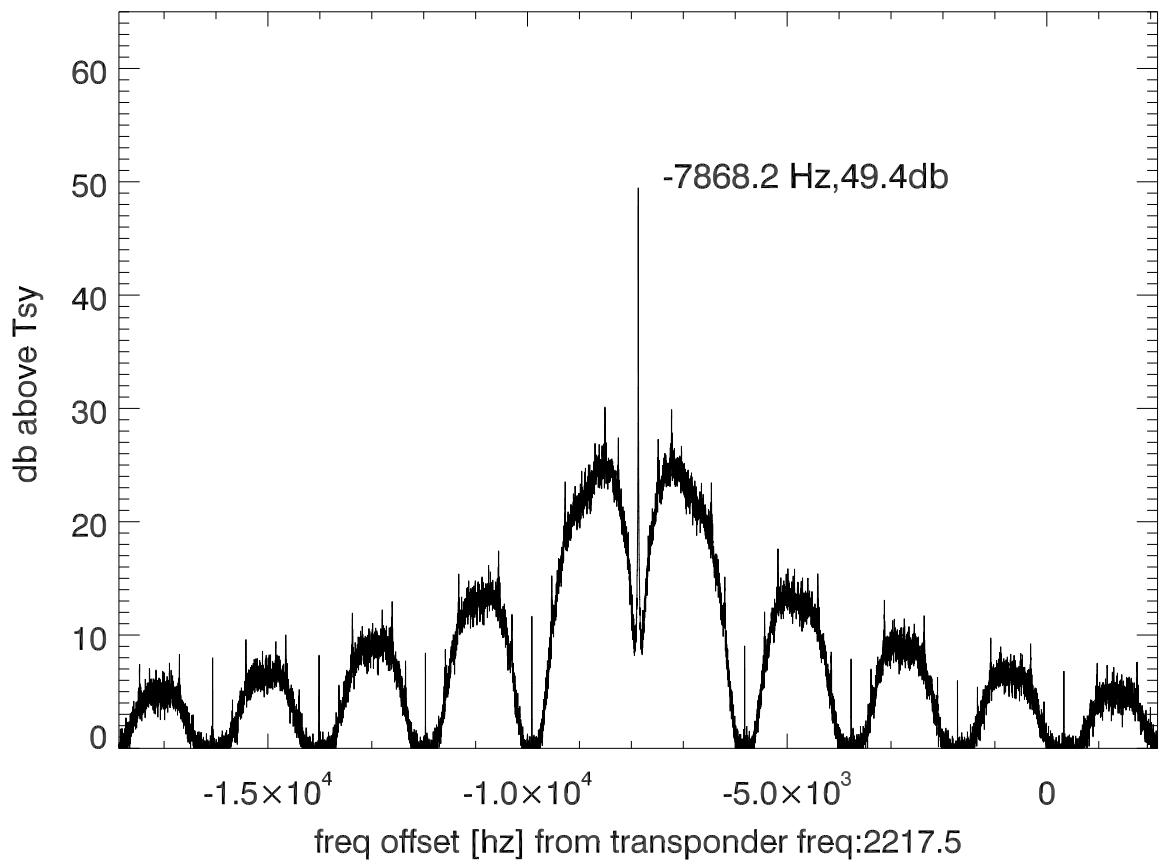
isee3 140624:185749 (UTC) spectra after doppler correction. PoIB
