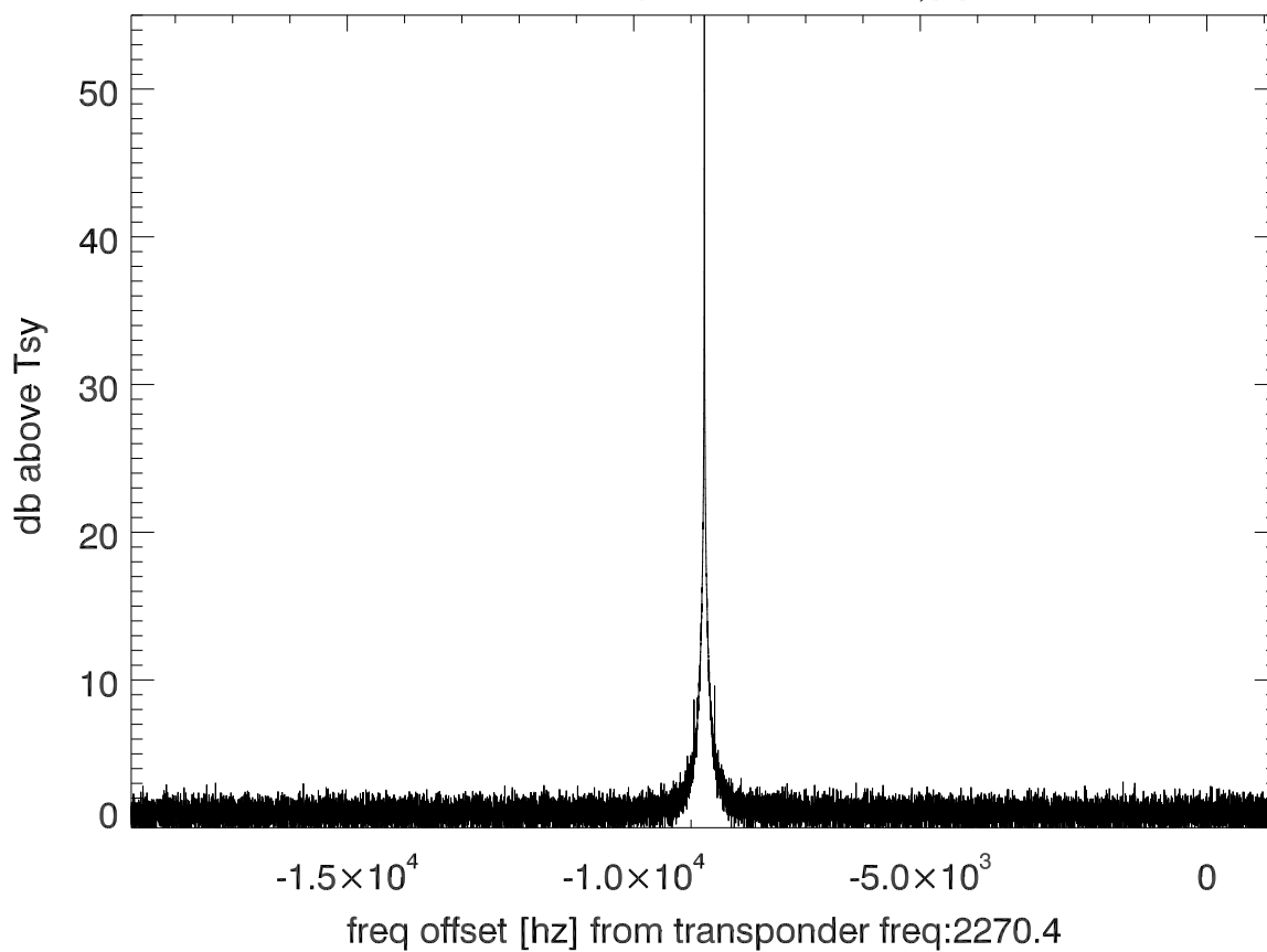
isee3 140620:190752 (UTC) spectra after doppler correction. PoIB
