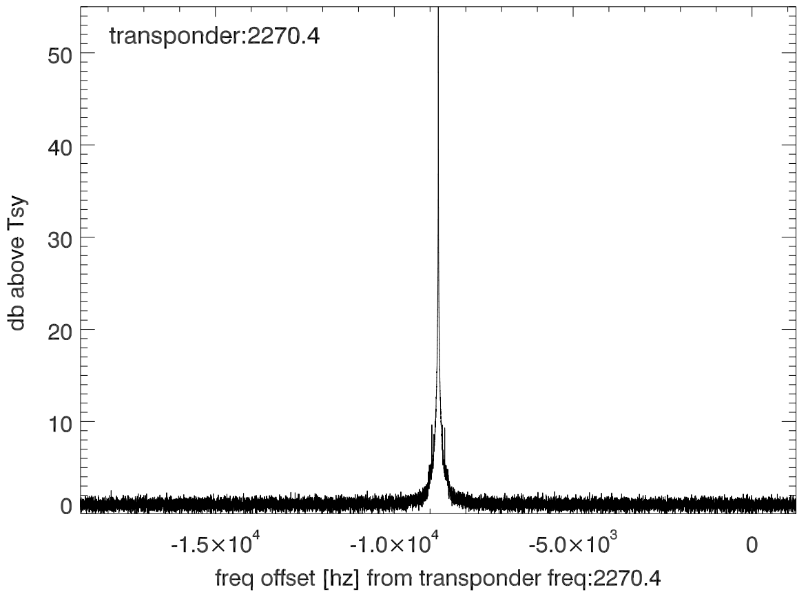
isee3 140620:181931 (UTC) spectra after doppler correction. PolA
