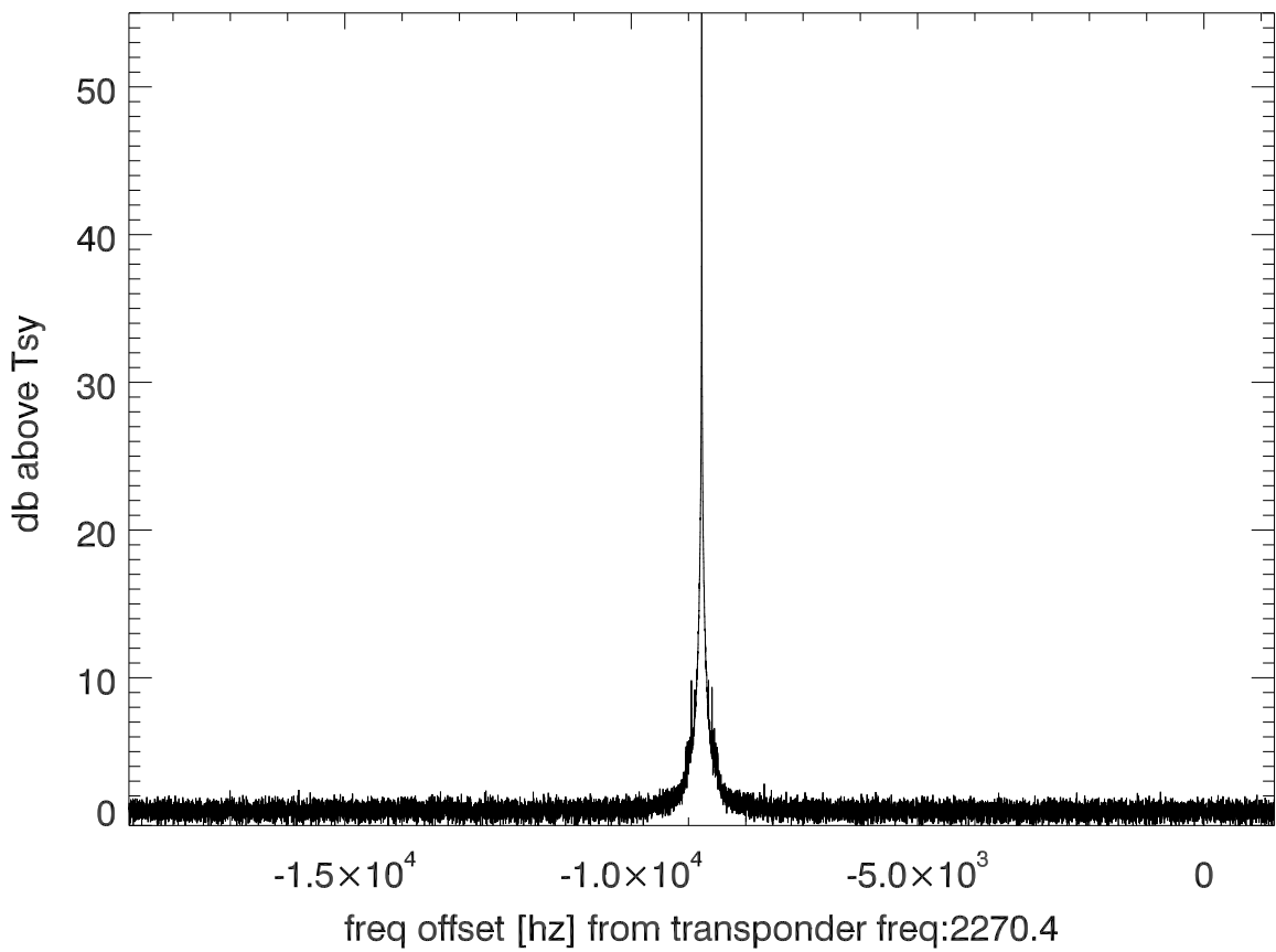
isee3 140620:181931 (UTC) spectra after doppler correction. PolB
