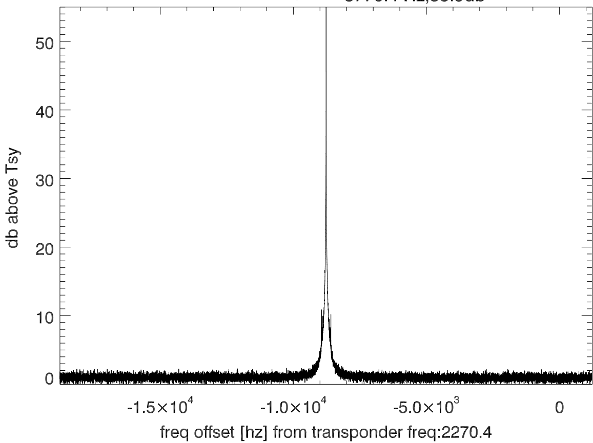
isee3 140620:180545 (UTC) spectra after doppler correction. PoIB
