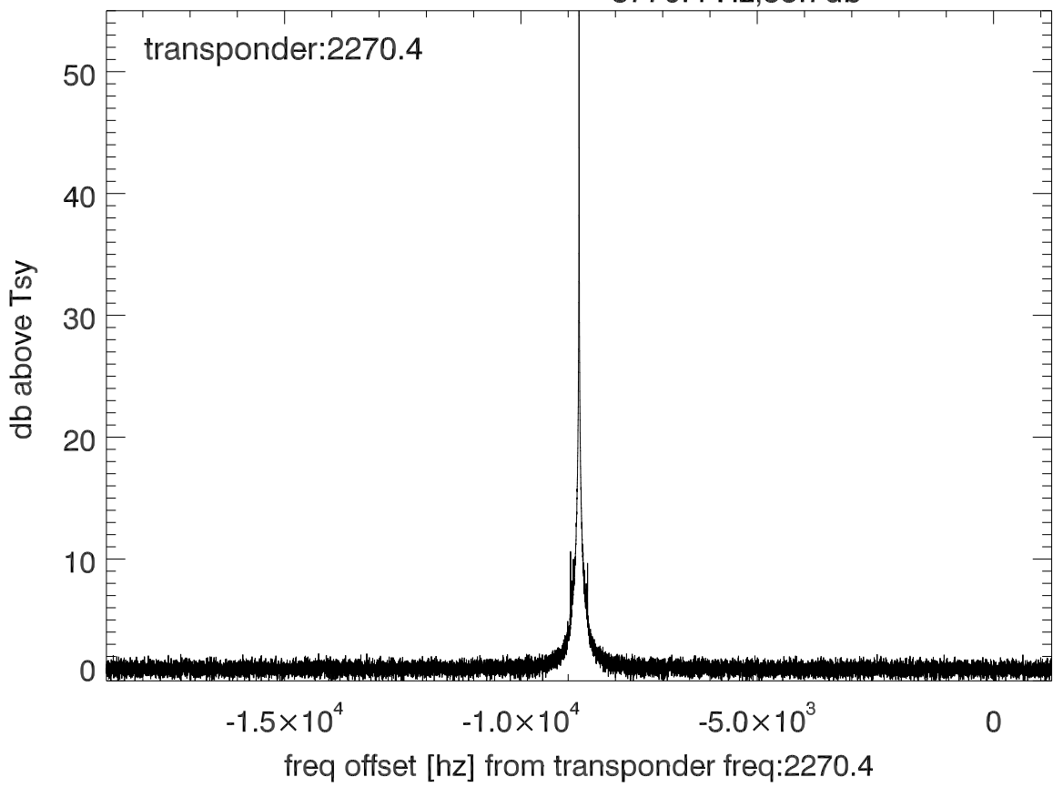
isee3 140620:180545 (UTC) spectra after doppler correction. PoIA
