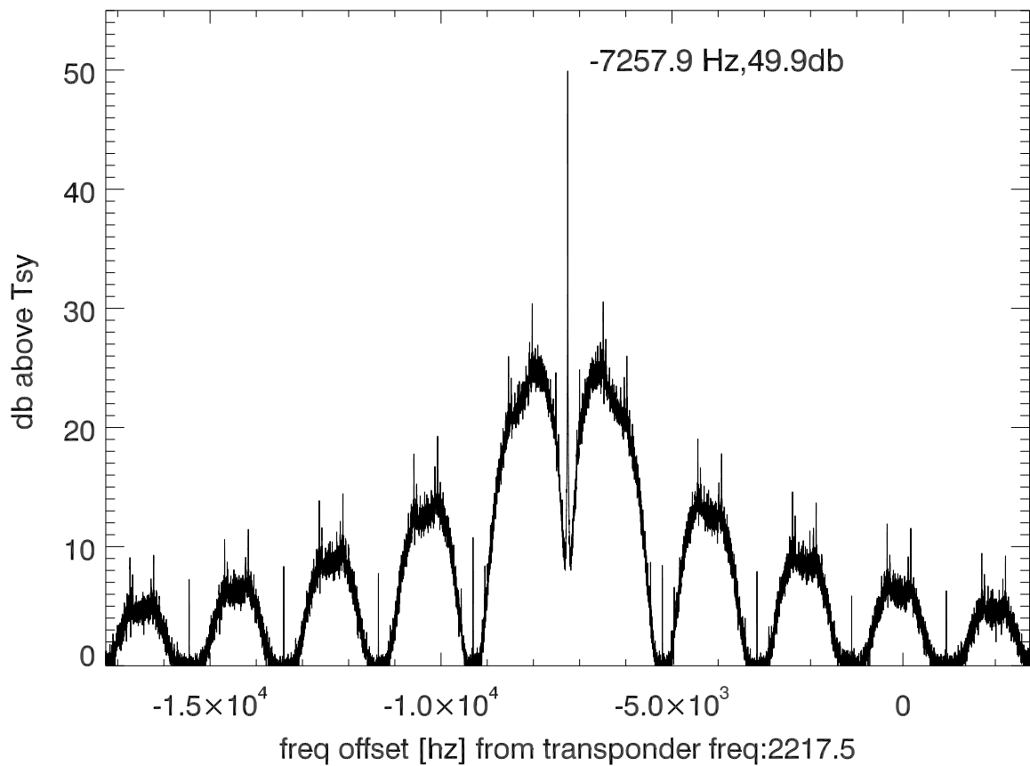
isee3 140620:193518 (UTC) spectra after doppler correction. PoIB
