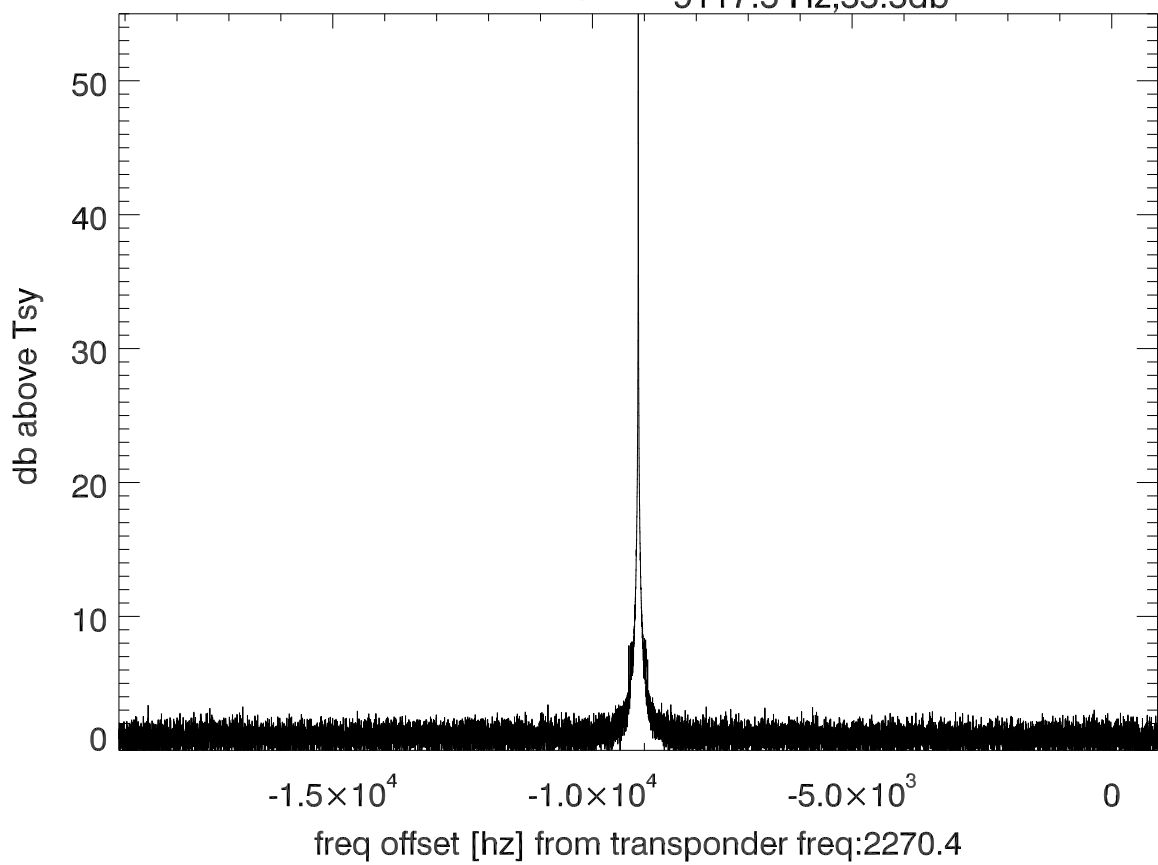
isee3 140615:190641 (UTC) spectra after doppler correction. PolB
