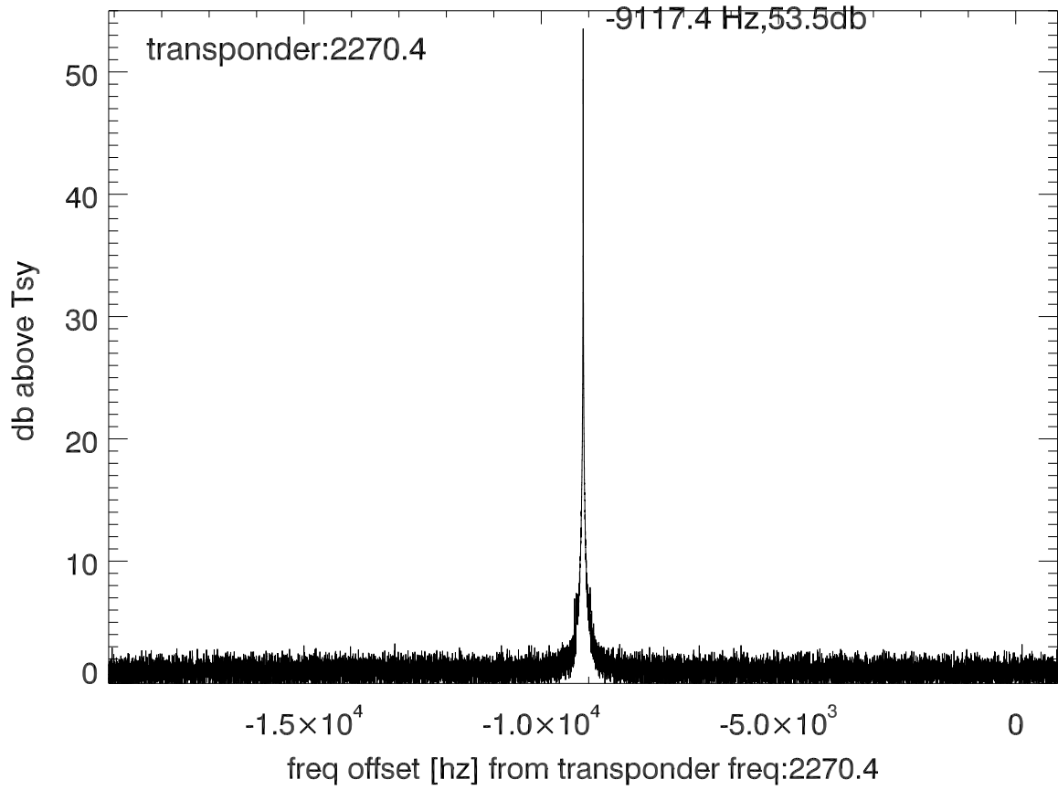
isee3 140615:190641 (UTC) spectra after doppler correction. PolA
