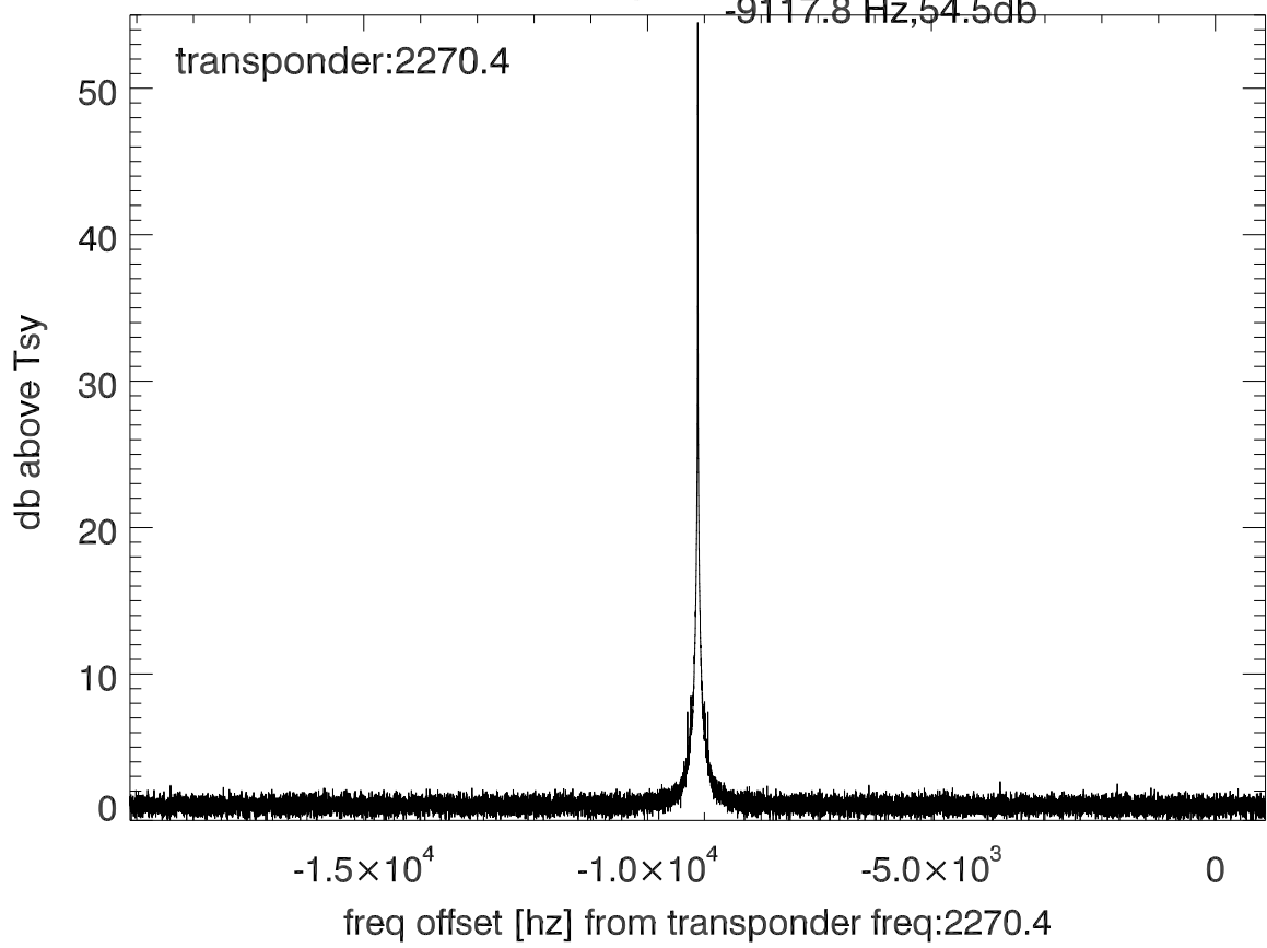
isee3 140615:185828 (UTC) spectra after doppler correction. PolA
