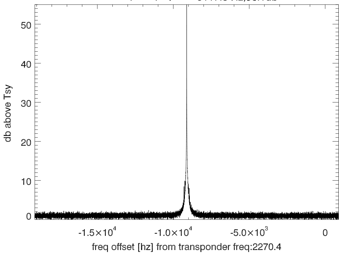
isee3 140615:185828 (UTC) spectra after doppler correction. PolB
