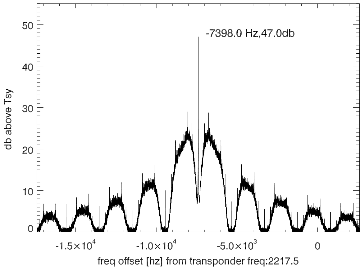
isee3 140615:191850 (UTC) spectra after doppler correction. PoIB
