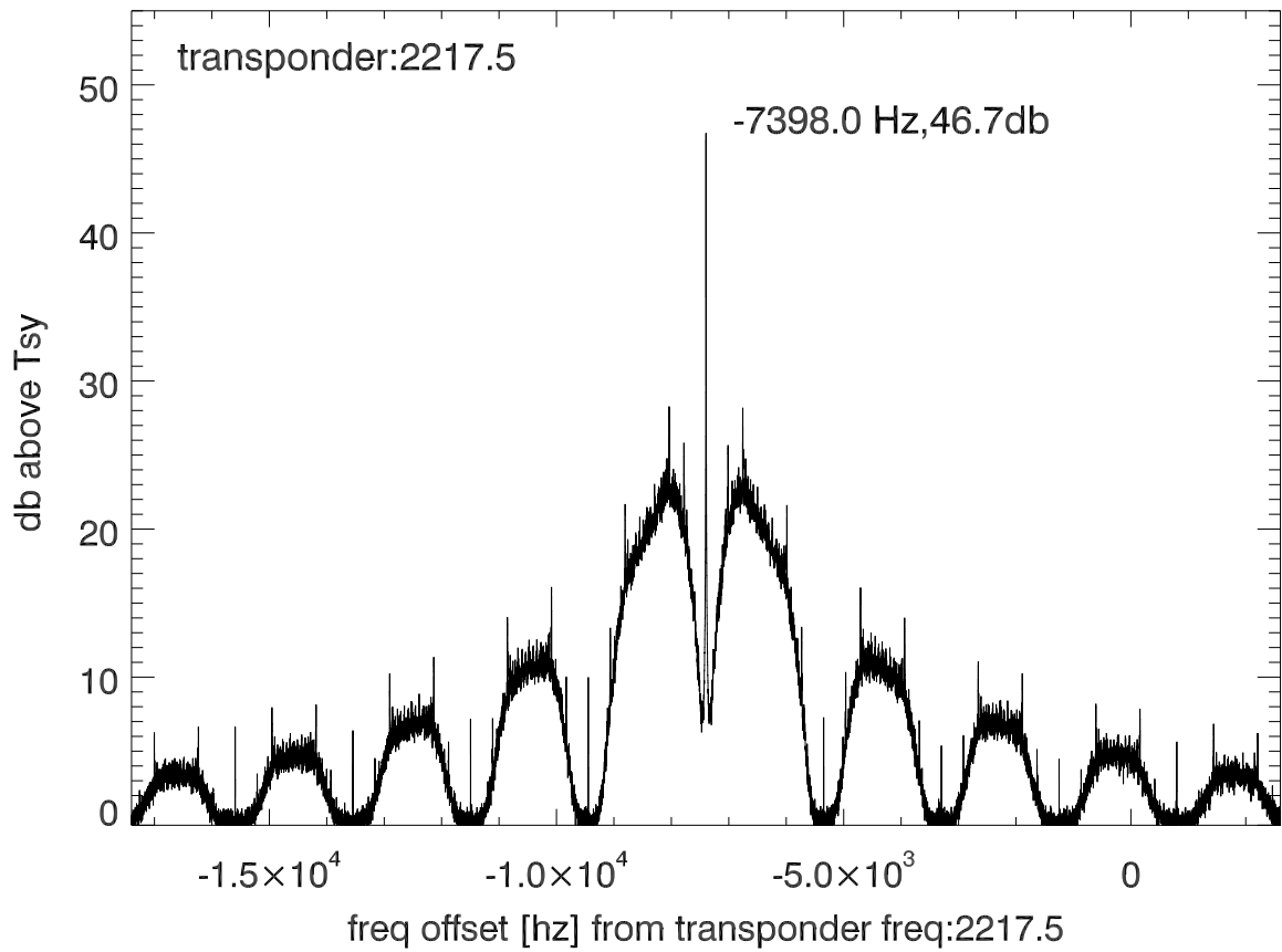
isee3 140615:191850 (UTC) spectra after doppler correction. PoIA
