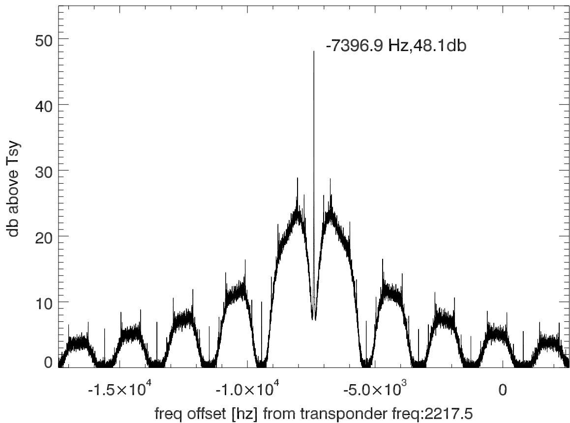
isee3 140615:201935 (UTC) spectra after doppler correction. PolB
