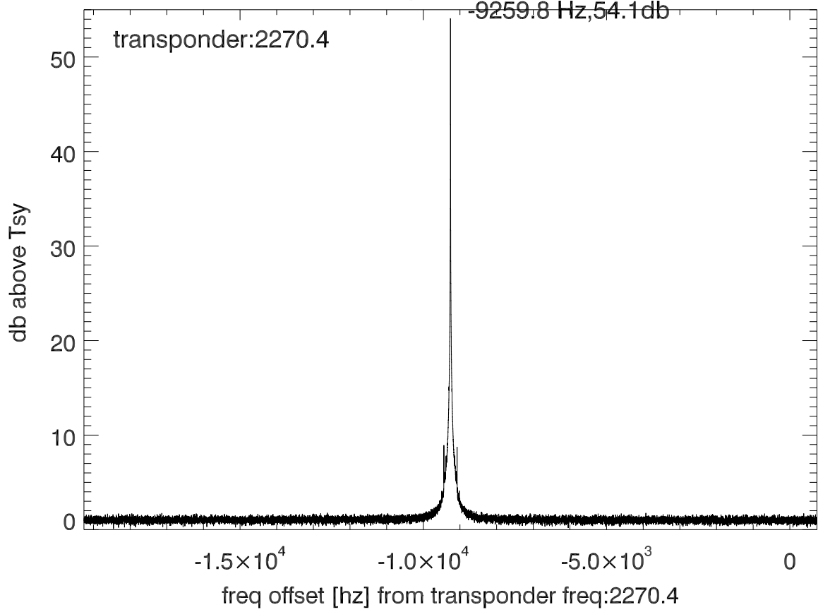
isee3 140613:200649 (UTC) spectra after doppler correction. PolA
