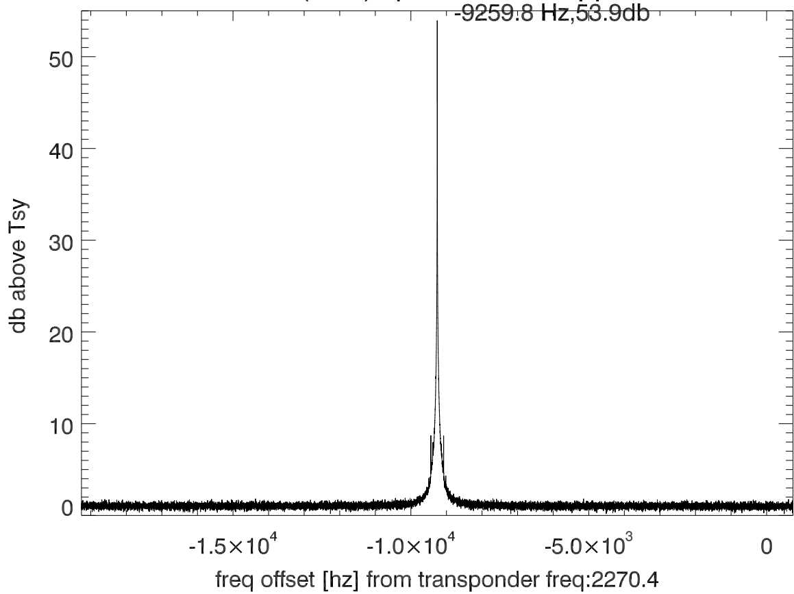
isee3 140613:200649 (UTC) spectra after doppler correction. PolB
