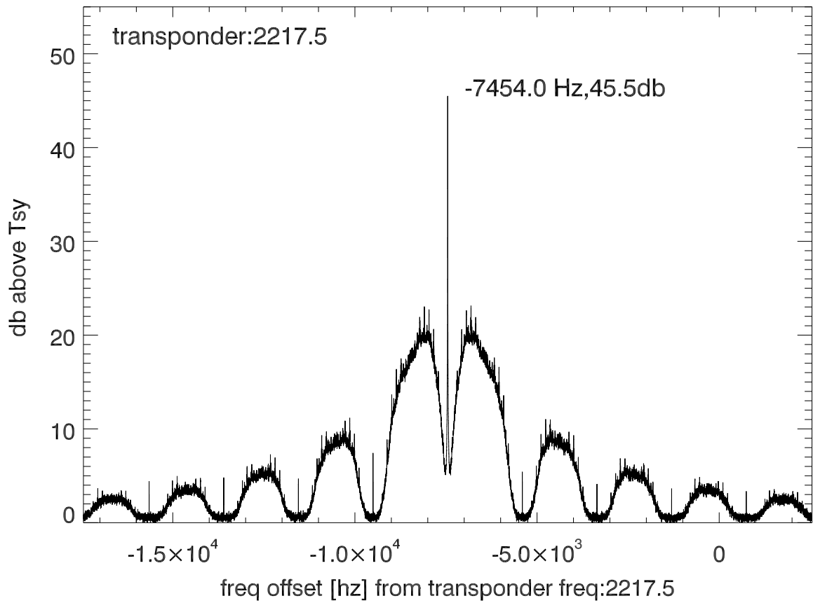
isee3 140613:203200 (UTC) spectra after doppler correction. PolA
