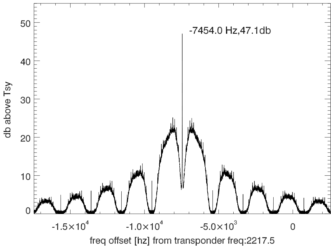
isee3 140613:203200 (UTC) spectra after doppler correction. PolB
